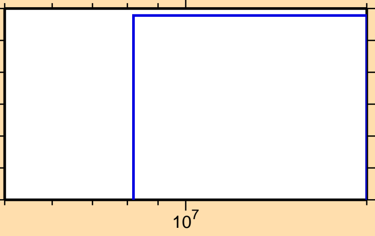
\sigma vs. E for ^{239}\text{Es}(n,2n)
