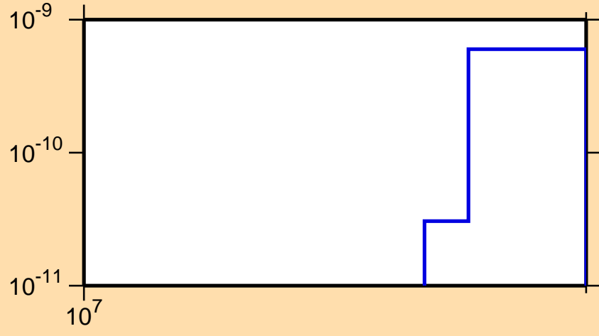
\sigma vs. E for ^{240}\text{Es}(n,3n)
