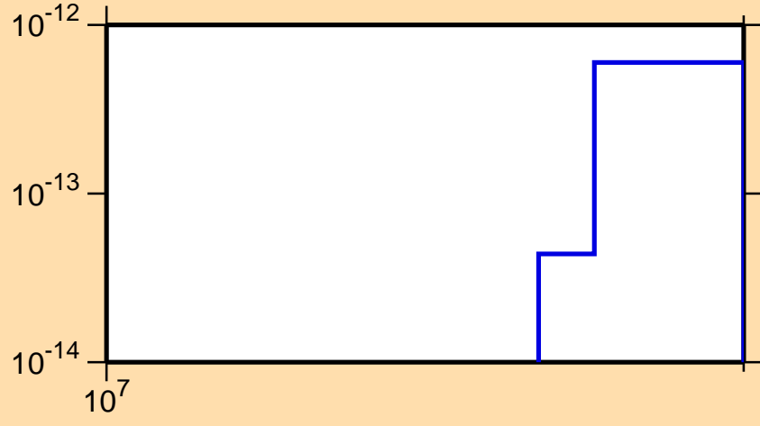
\sigma vs. E for ^{240}\text{Es} (mt 34)
