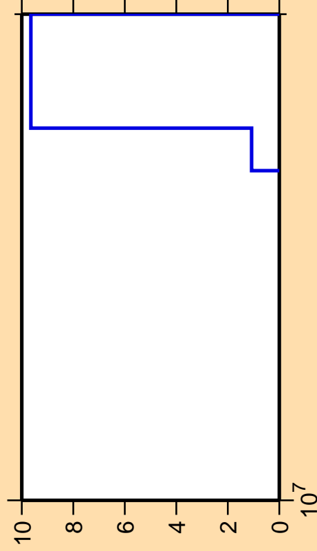
\Delta\sigma/\sigma vs. E for ^{240}\text{Es}(n,pd)
