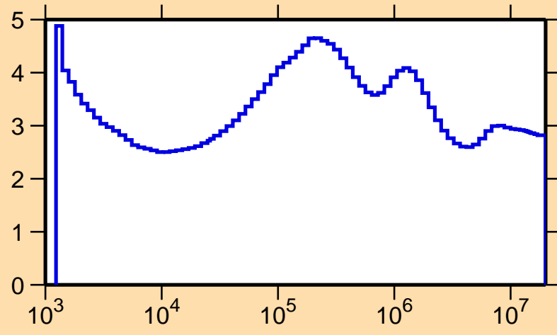
\sigma vs. E for ^{240}\text{Es}(n,\text{nonel.})
