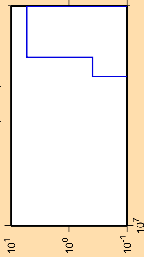
\Delta\sigma/\sigma vs. E for ^{240}\text{Es} (mt 34)
