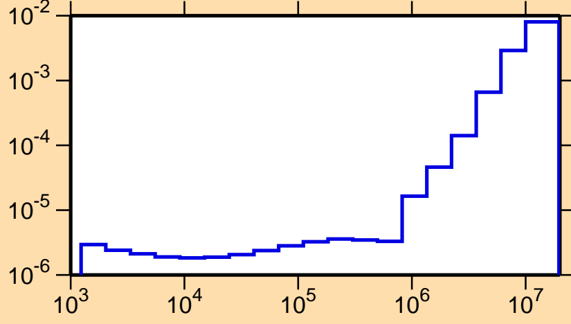
\sigma vs. E for ^{240}\text{Es}(n,p\alpha)
