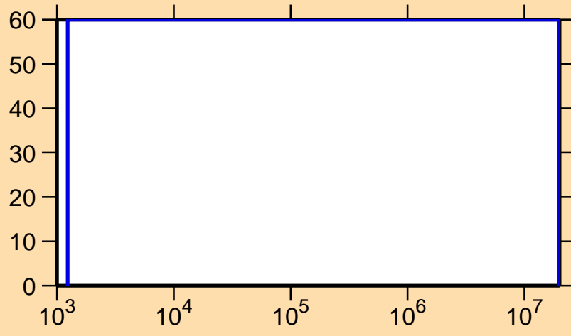
\Delta\sigma/\sigma vs. E for ^{240}\text{Es}(n,p)
