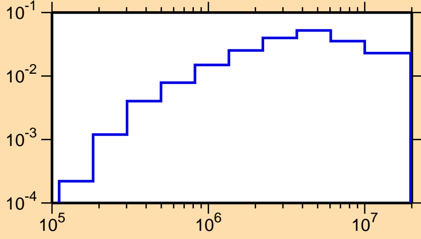
\sigma vs. E for ^{240}\text{Es}(n,\text{inel.})
