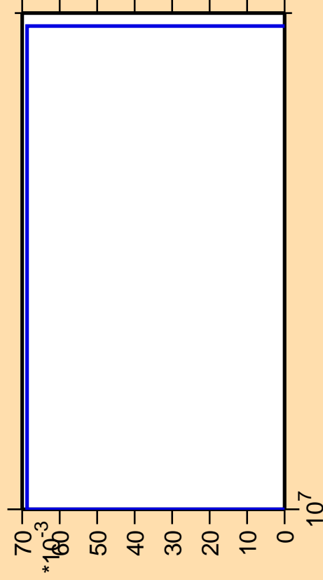
\Delta\sigma/\sigma vs. E for ^{240}\text{Es} (mt 34)
