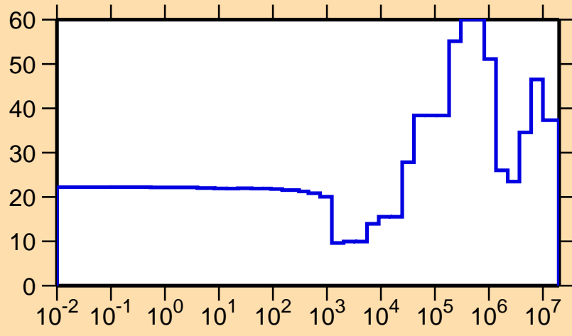
\Delta\sigma/\sigma vs. E for ^{240}\text{Es}(n,el.)
