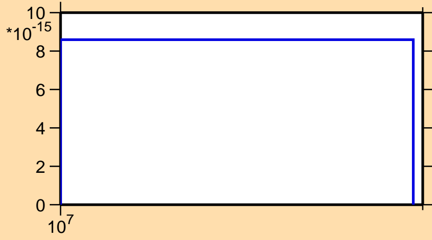
\sigma vs. E for ^{240}\text{Es} (mt 34)
