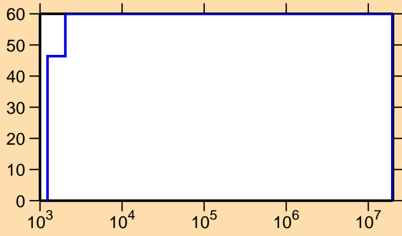
\Delta\sigma/\sigma vs. E for ^{240}\text{Es}(n,\gamma)
