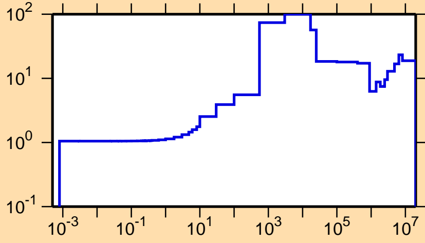
\Delta\sigma/\sigma vs. E for ^{240}\text{Es}(n,\text{tot.})
