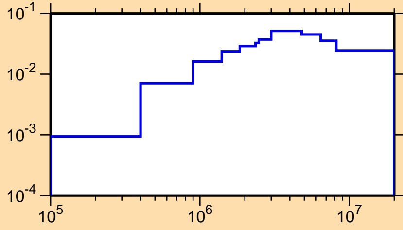
\sigma vs. E for ^{240}\text{Es}(n,n\text{cont.})
