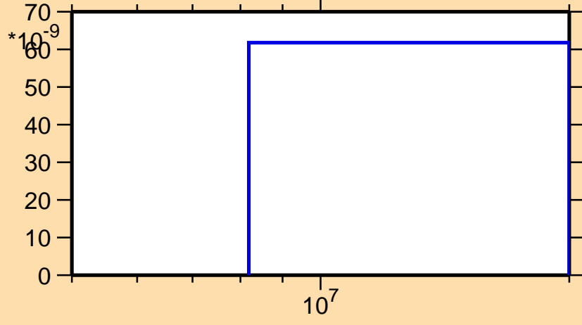
\sigma vs. E for ^{240}\text{Es}(n,\text{He3})
