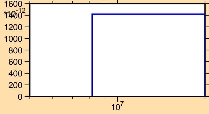
\sigma vs. E for ^{240}\text{Es}(n,2np)
