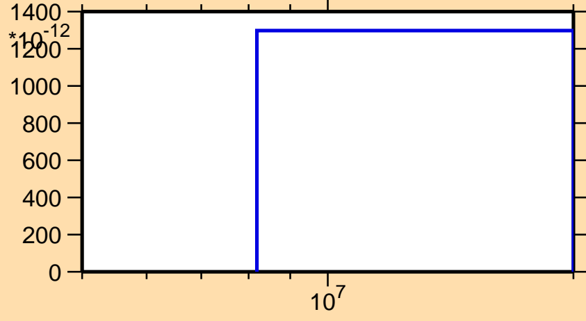
\sigma vs. E for ^{240}\text{Es}(n,nd)
