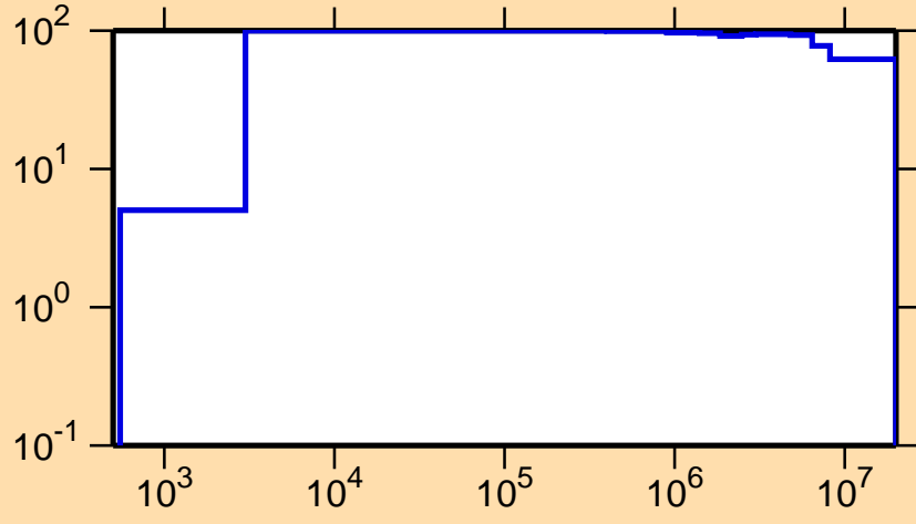
\Delta\sigma/\sigma vs. E for ^{240}\text{Es}(n,\gamma)
