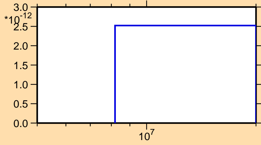
\sigma vs. E for ^{240}\text{Es}(n,nt)
