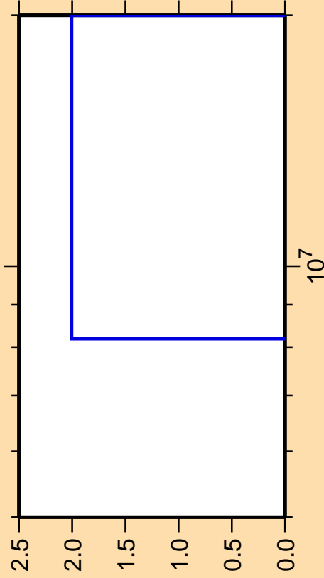
\Delta\sigma/\sigma vs. E for ^{240}\text{Es}(n,nt)
