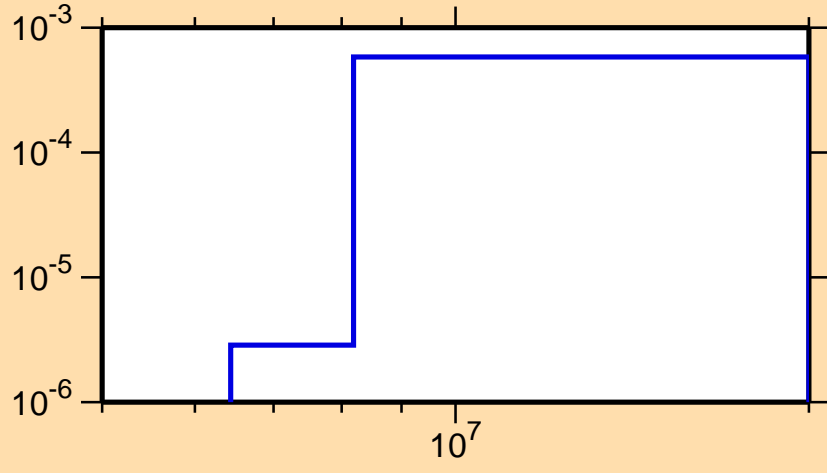
\sigma vs. E for ^{240}\text{Es}(n,2n)
