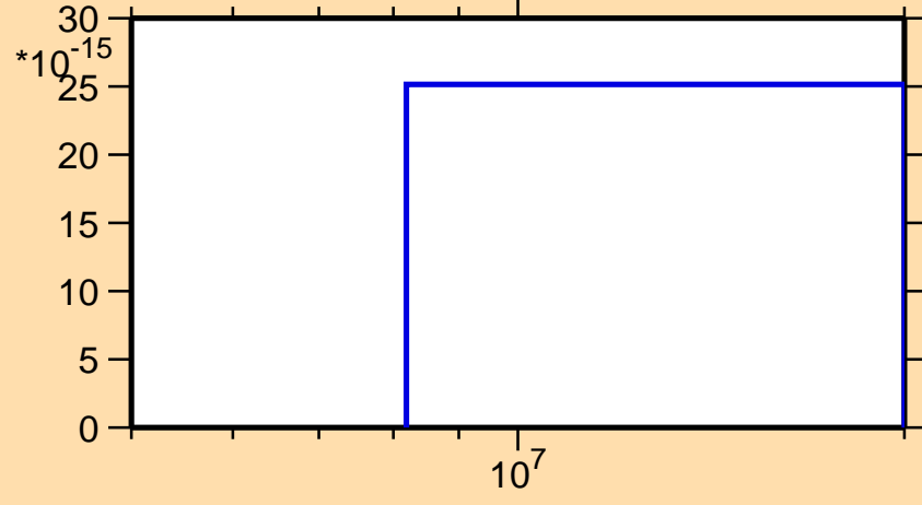
\sigma vs. E for ^{240}\text{Es}(n,pd)
