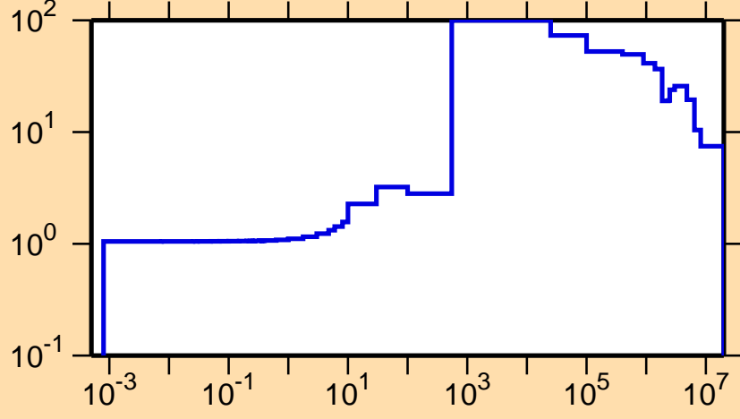
\Delta\sigma/\sigma vs. E for ^{240}\text{Es}(n,f)
