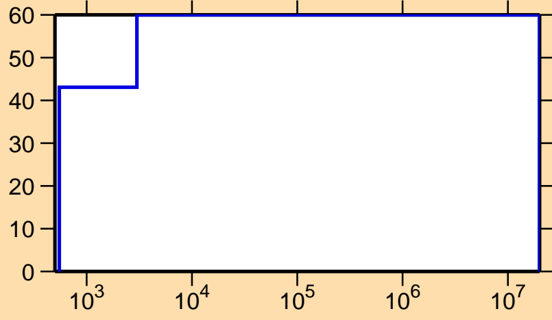
\Delta\sigma/\sigma vs. E for ^{240}\text{Es}(n,p)
