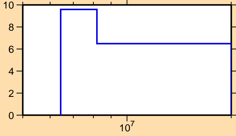
\Delta\sigma/\sigma vs. E for ^{240}\text{Es}(n,\text{nonel.})
