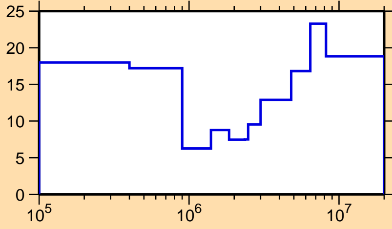
\Delta\sigma/\sigma vs. E for ^{240}\text{Es}(n,\text{tot.})
