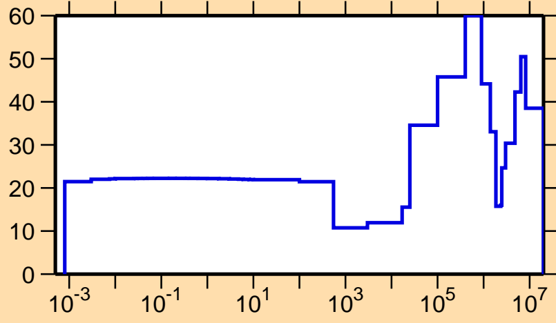
\Delta\sigma/\sigma vs. E for ^{240}\text{Es}(n,\text{el.})
