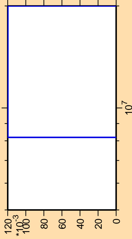
\Delta\sigma/\sigma vs. E for ^{240}\text{Es}(n,pd)
