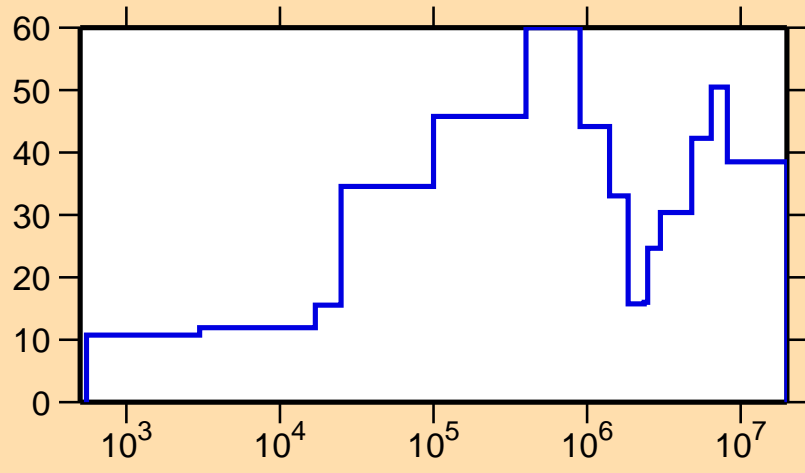
\Delta\sigma/\sigma vs. E for ^{240}\text{Es}(n,\text{el.})
