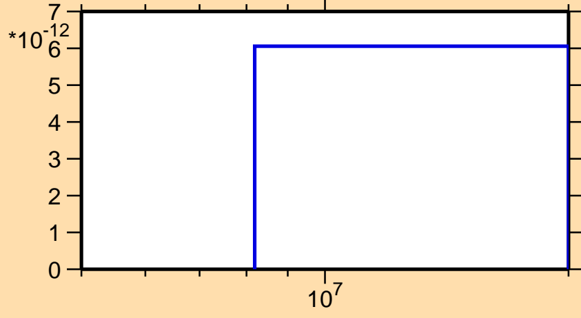
\sigma vs. E for ^{240}\text{Es}(n,3n)
