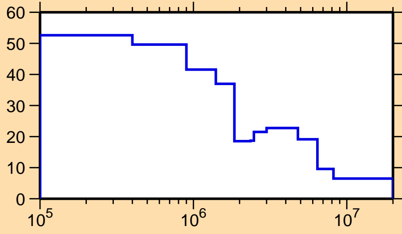
\Delta\sigma/\sigma vs. E for ^{240}\text{Es}(n,\text{nonel.})
