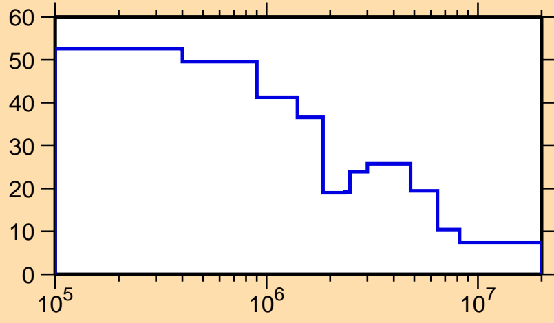
\Delta\sigma/\sigma vs. E for ^{240}\text{Es}(n,f)
