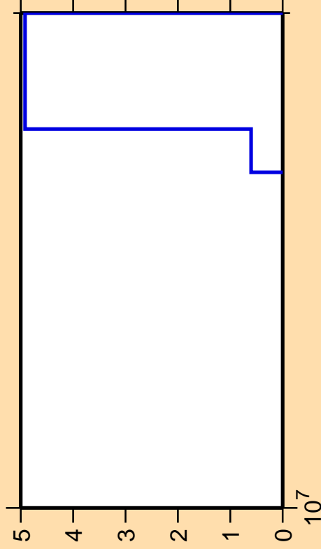
\Delta\sigma/\sigma vs. E for ^{241}\text{Es}(n,pd)
