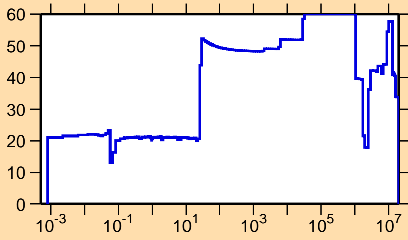
\Delta\sigma/\sigma vs. E for ^{241}\text{Es}(n,el.)
