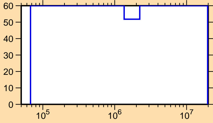
\Delta\sigma/\sigma vs. E for ^{241}\text{Es}(n,n_1)
