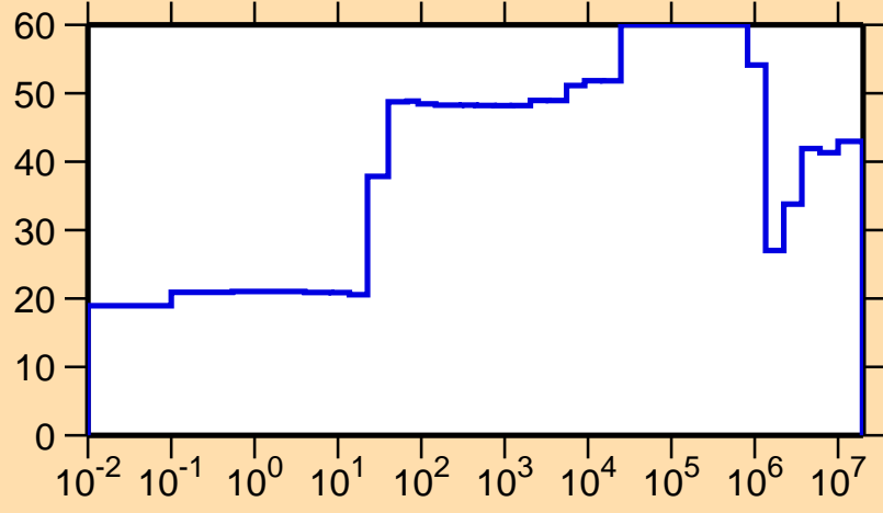
\Delta\sigma/\sigma vs. E for ^{241}\text{Es}(n,el.)
