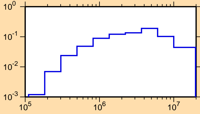
\sigma vs. E for ^{241}\text{Es}(n,n\text{cont.})
