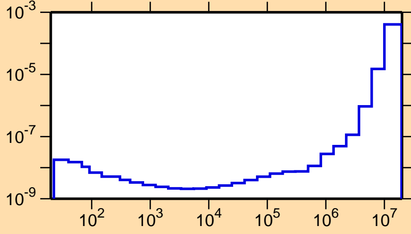
\sigma vs. E for ^{241}\text{Es}(n,p\alpha)
