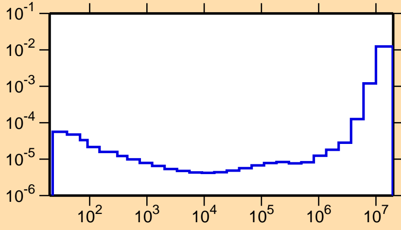
\sigma vs. E for ^{241}\text{Es}(n,p)
