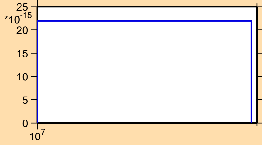
\sigma vs. E for ^{241}\text{Es}(n,pd)
