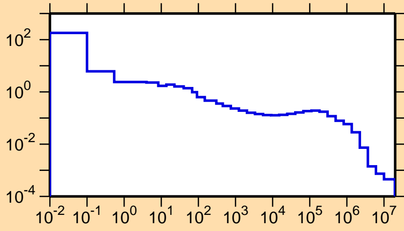
\sigma vs. E for ^{241}\text{Es}(n,\gamma)
