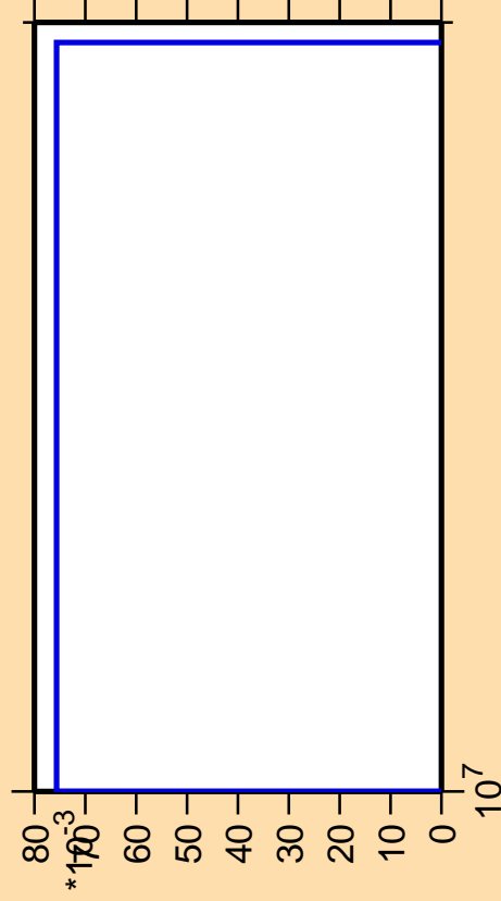
\Delta\sigma/\sigma vs. E for ^{241}\text{Es}(n,pd)
