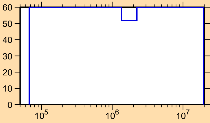
\Delta\sigma/\sigma vs. E for ^{241}\text{Es}(n,n_1)
