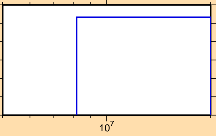
\sigma vs. E for ^{241}\text{Es}(n,2np)
