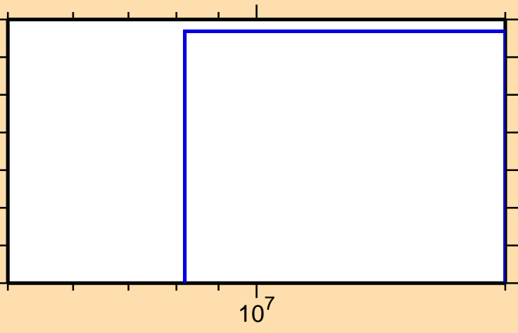
\sigma vs. E for ^{241}\text{Es}(n,\text{He3})
