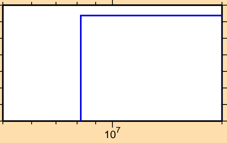
\sigma vs. E for ^{241}\text{Es}(n,nt)
