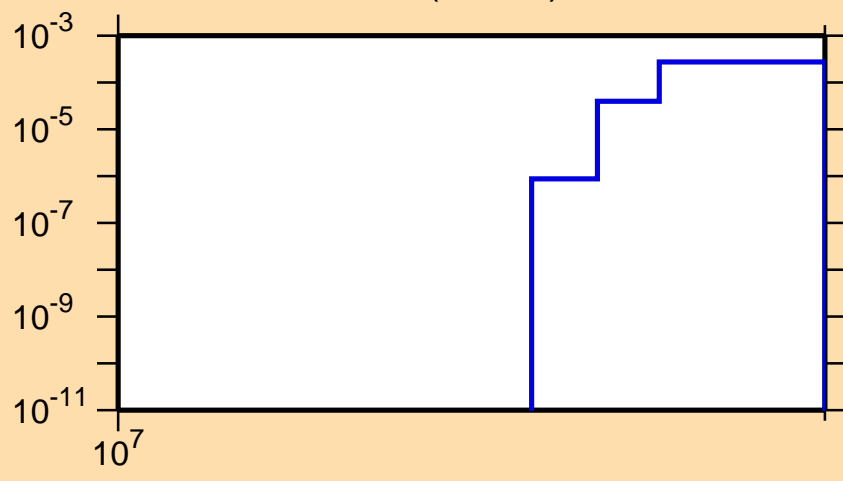
\sigma vs. E for ^{242}\text{Es}(n,3n\alpha)
