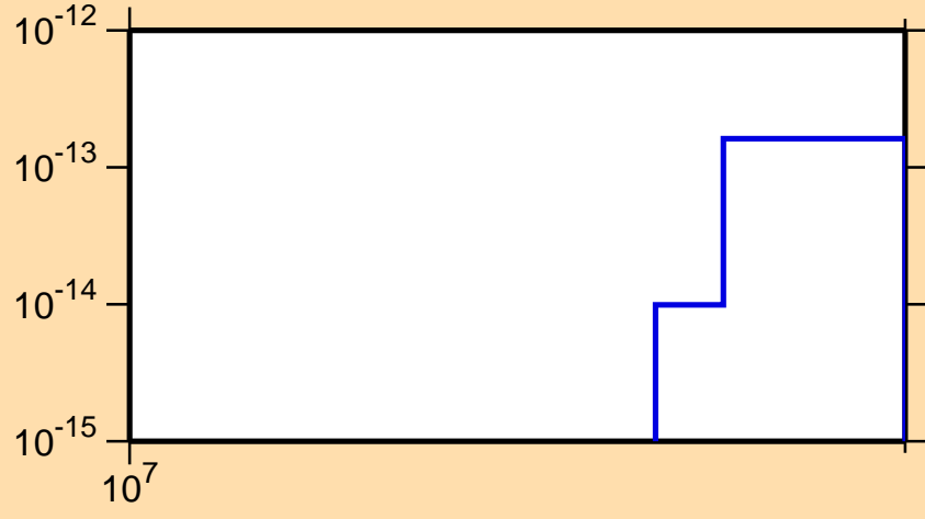
\sigma vs. E for ^{242}\text{Es}(n,pt)
