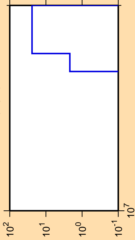
\Delta\sigma/\sigma vs. E for ^{242}\text{Es}(n,\text{pd})
