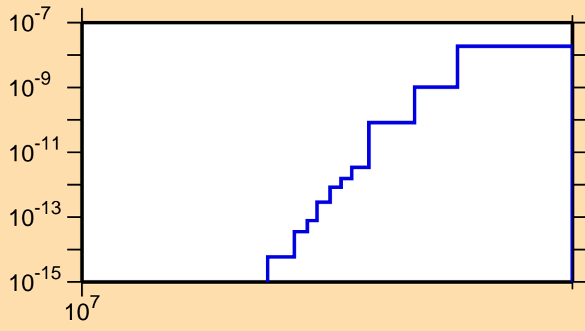
\sigma vs. E for ^{242}\text{Es}(n,nt)
