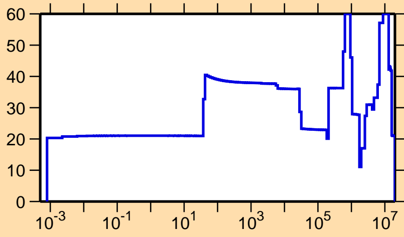
\Delta\sigma/\sigma vs. E for ^{242}\text{Es}(n,el.)
