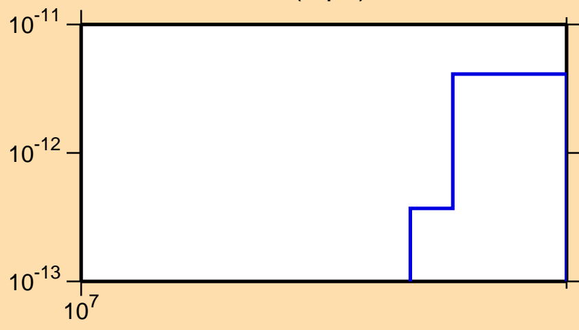
\sigma vs. E for ^{242}\text{Es}(n,\text{pd})
