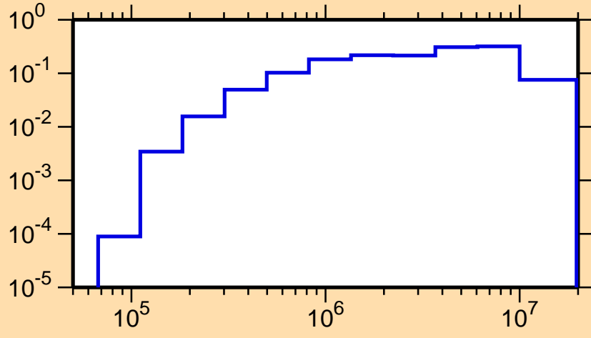
\sigma vs. E for ^{242}\text{Es}(n,n\alpha)
