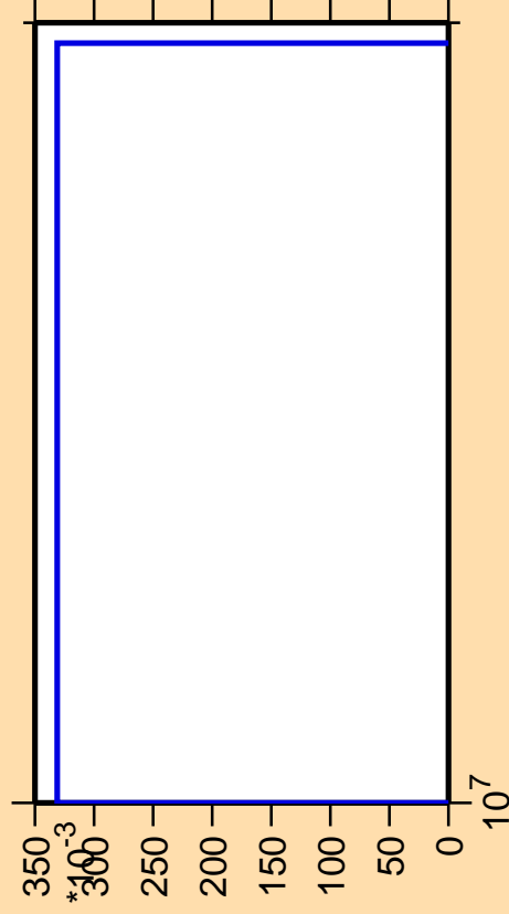
\Delta\sigma/\sigma vs. E for ^{242}\text{Es}(n,pd)
