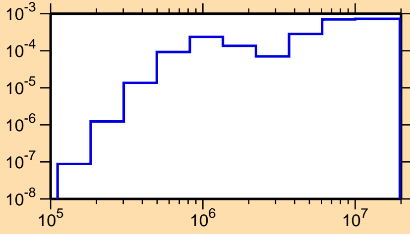
\sigma vs. E for ^{242}\text{Es}(n,n_1)
