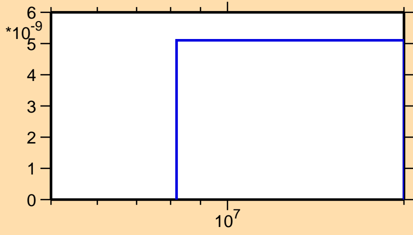
\sigma vs. E for ^{243}\text{Es}(n,\text{He3})
