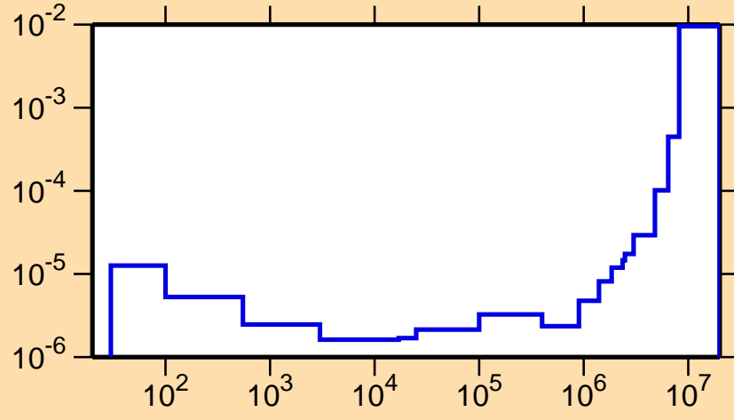
\sigma vs. E for ^{243}\text{Es}(n,p)
