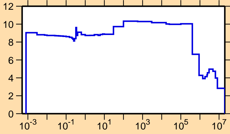
\sigma vs. E for ^{243}\text{Es}(n,\text{el.})
