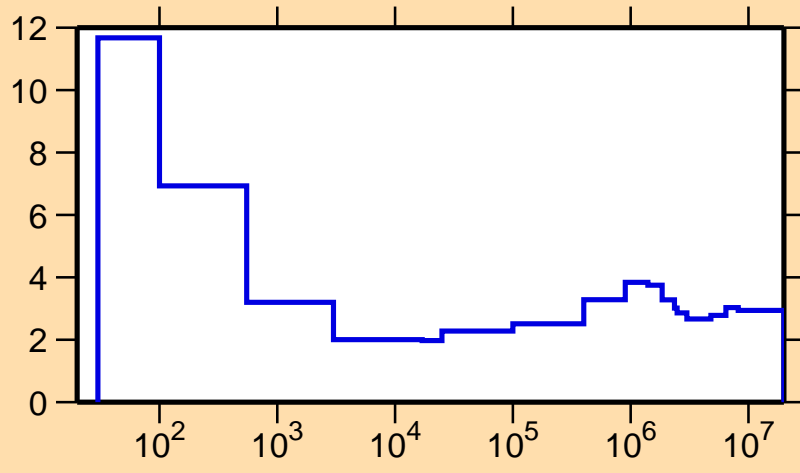
\sigma vs. E for ^{243}\text{Es}(n,\text{nonel.})
