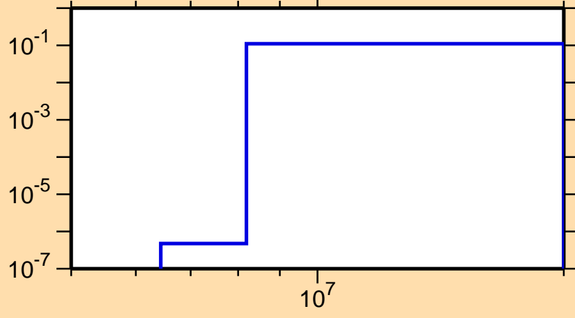
\sigma vs. E for ^{243}\text{Es}(n,2n)
