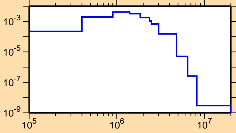
\sigma vs. E for ^{243}\text{Es}(n,n_4)
