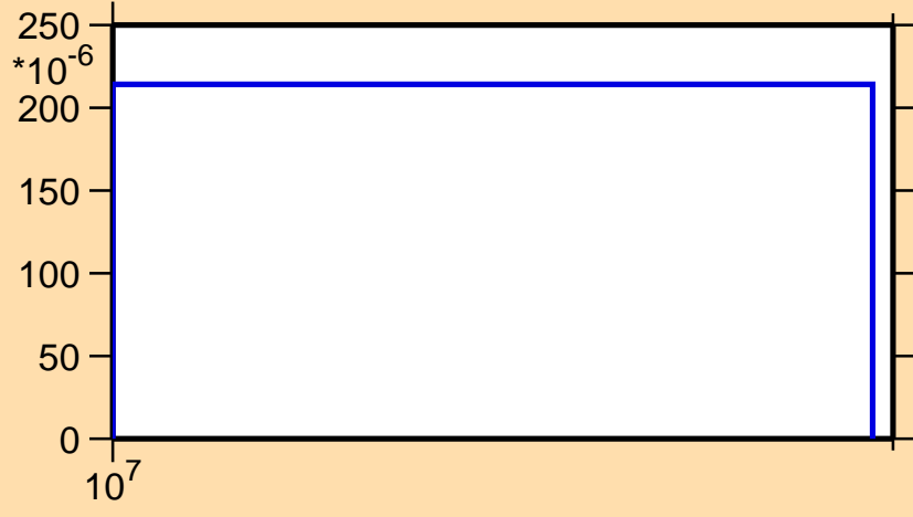
\sigma vs. E for ^{244}\text{Es}(n,3n\alpha)
