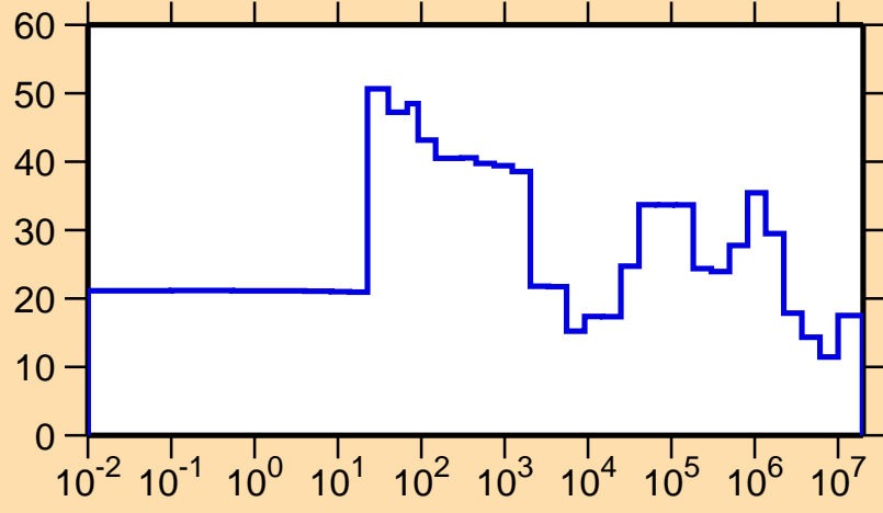
\Delta\sigma/\sigma vs. E for ^{244}\text{Es}(n,el.)
