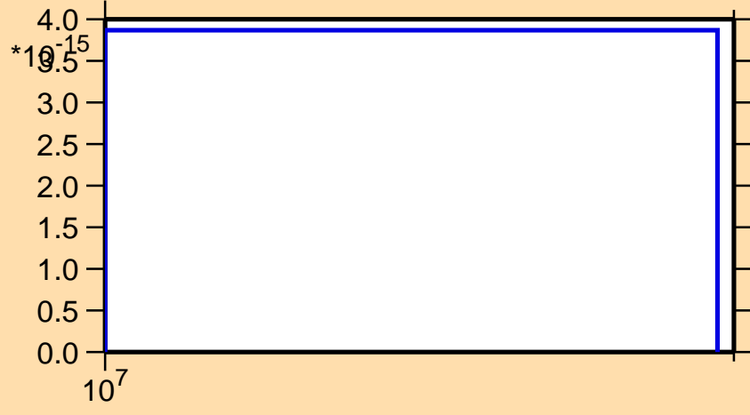
\sigma vs. E for ^{244}\text{Es}(n,pt)
