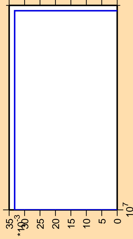
\Delta\sigma/\sigma vs. E for ^{244}\text{Es}(n,pt)
