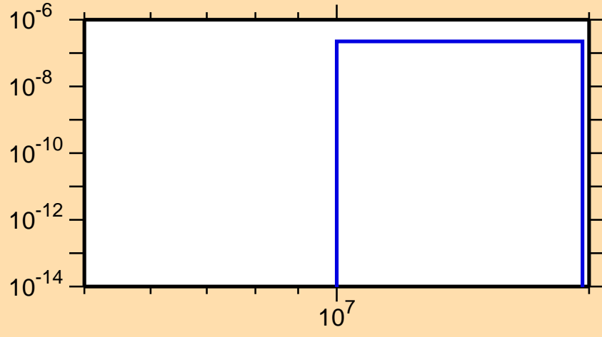
\sigma vs. E for ^{244}\text{Es}(n,2np)
