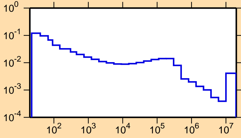
\sigma vs. E for ^{244}\text{Es}(n,\alpha)
