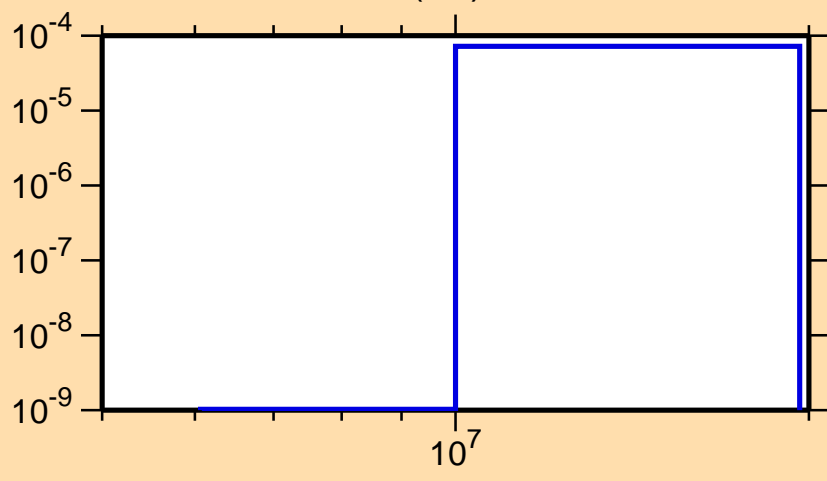
\sigma vs. E for ^{244}\text{Es}(n,t)
