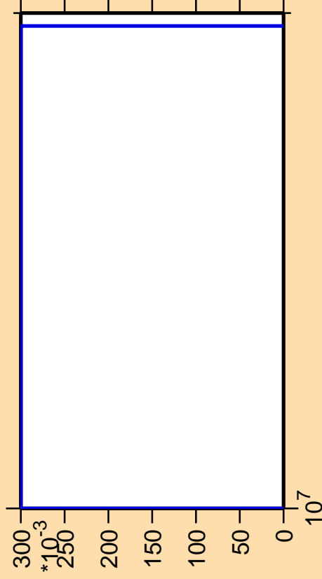
\Delta\sigma/\sigma vs. E for ^{244}\text{Es} (mt 34)
