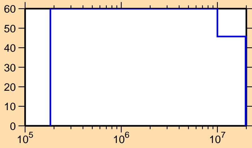
\Delta\sigma/\sigma vs. E for ^{244}\text{Es}(n,n_1)
