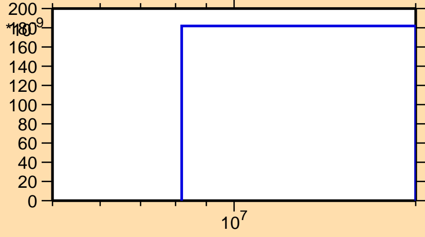
\sigma vs. E for ^{244}\text{Es}(n,2np)
