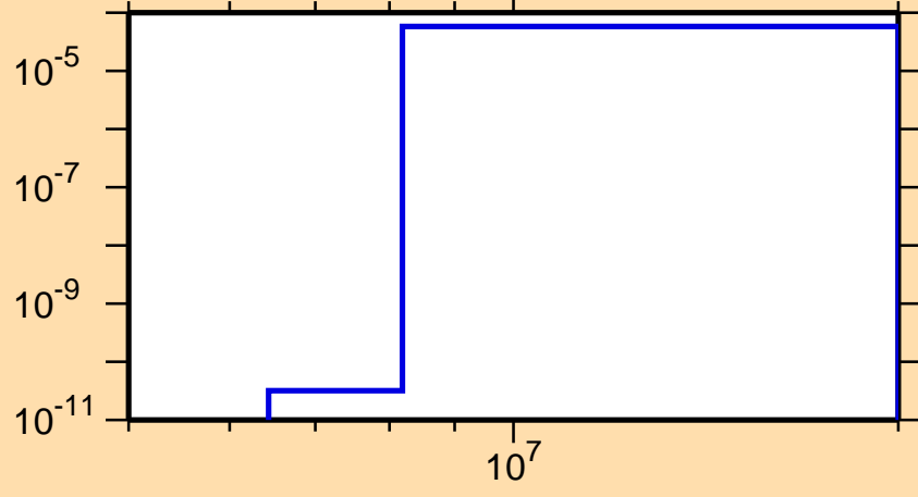
\sigma vs. E for ^{244}\text{Es}(n,t)
