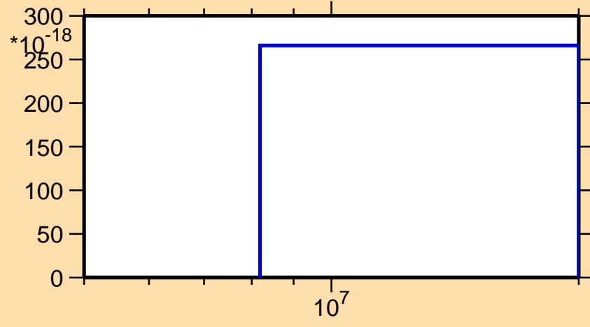
\sigma vs. E for ^{244}\text{Es} (mt 11)
