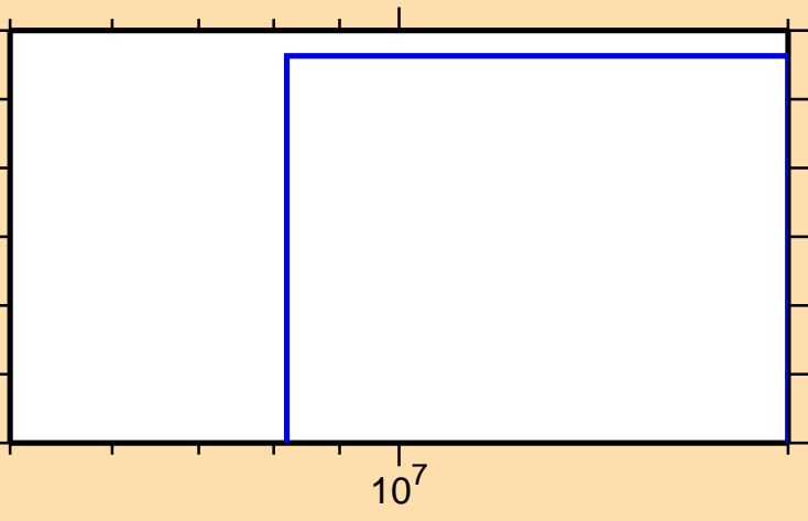
\sigma vs. E for ^{244}\text{Es}(n,\text{He3})
