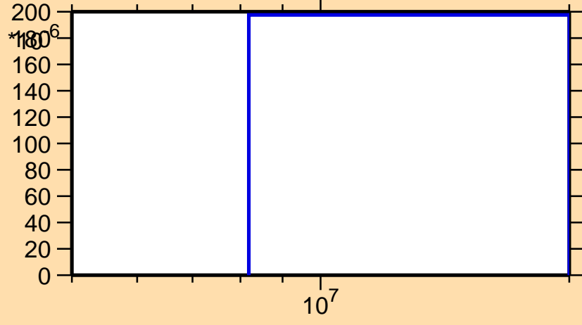
\sigma vs. E for ^{244}\text{Es}(n,3n)
