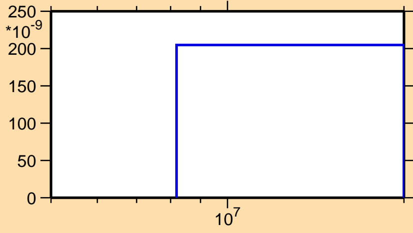
\sigma vs. E for ^{244}\text{Es}(n,nd)
