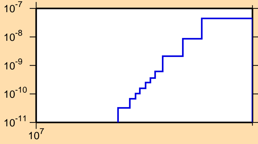
\sigma vs. E for ^{245}\text{Es}(n,\text{He3})
