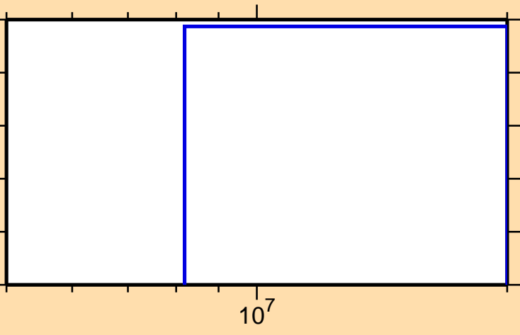
\sigma vs. E for ^{245}\text{Es} (mt 34)
