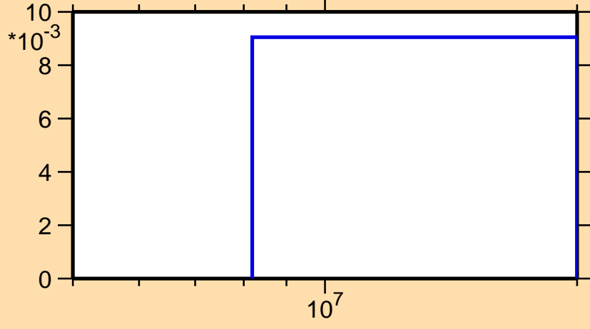
\sigma vs. E for ^{245}\text{Es}(n,3n)
