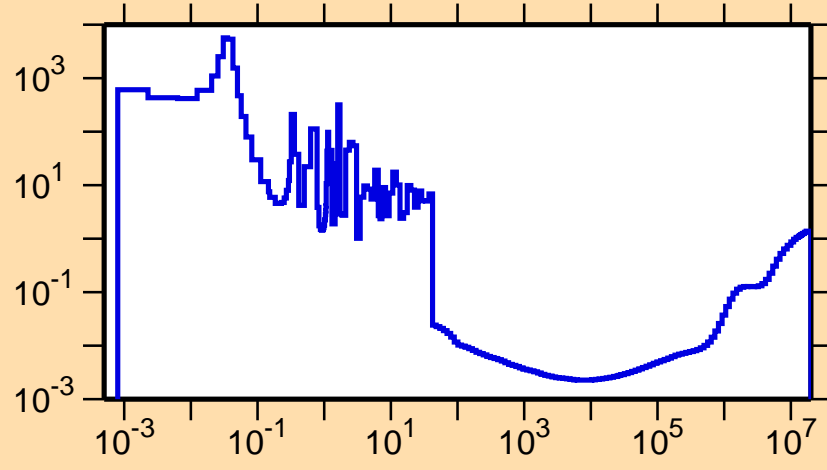
\sigma vs. E for ^{246}\text{Es}(n,f)
