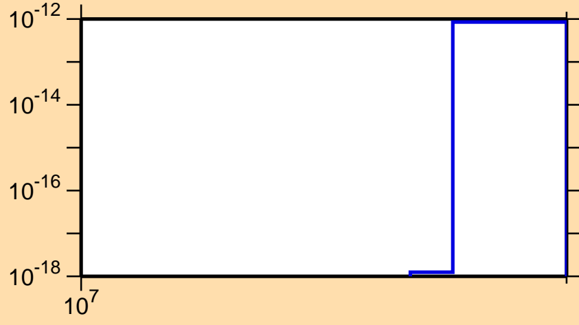
\sigma vs. E for ^{246}\text{Es} (mt 11)
