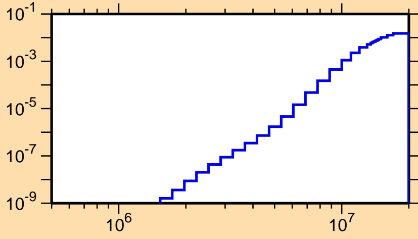
\sigma vs. E for ^{246}\text{Es}(n,p\alpha)
