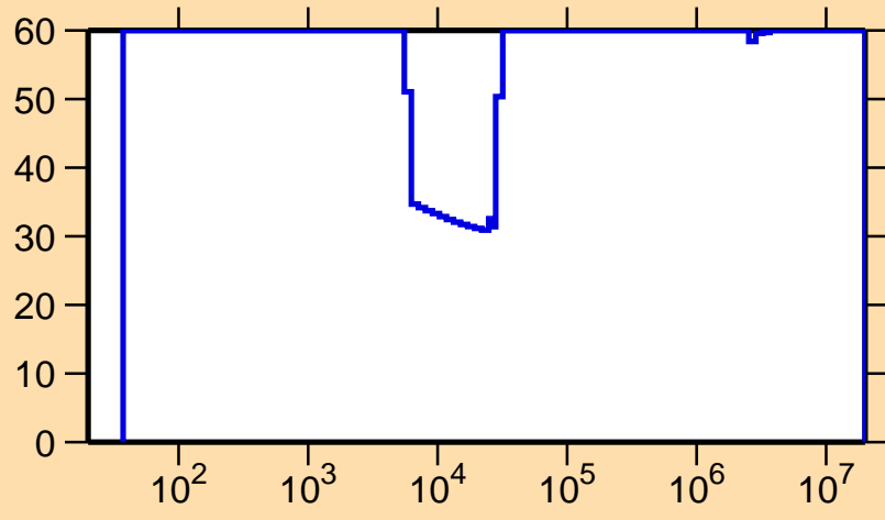
\Delta\sigma/\sigma vs. E for ^{246}\text{Es}(n,\gamma)
