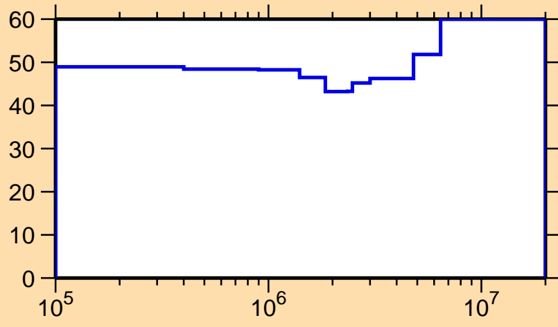
\Delta\sigma/\sigma vs. E for ^{246}\text{Es}(n,\text{inel.})
