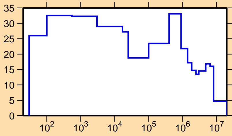
\Delta\sigma/\sigma vs. E for ^{246}\text{Es}(n,\text{el.})
