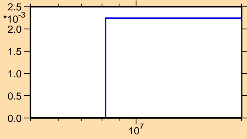
\sigma vs. E for ^{246}\text{Es}(n,3n\alpha)
