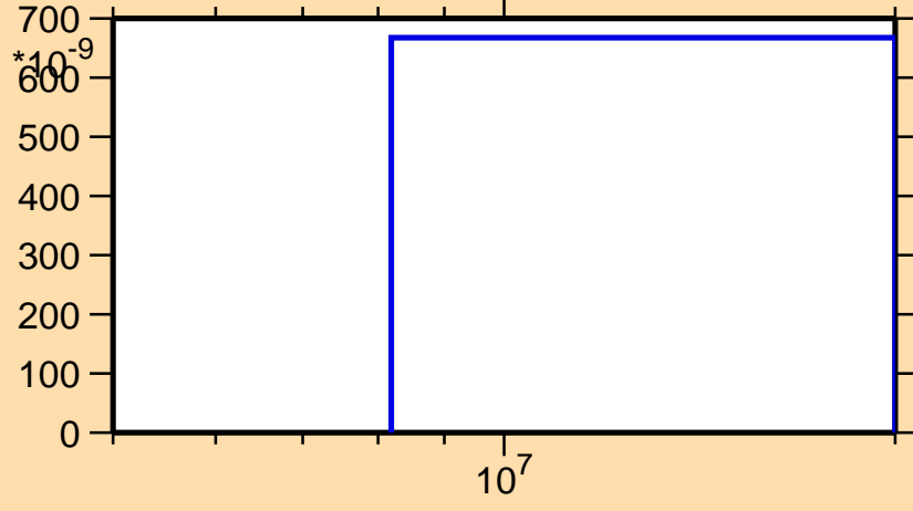
\sigma vs. E for ^{246}\text{Es}(n,nd)
