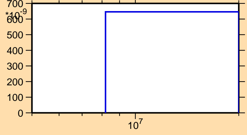
\sigma vs. E for ^{246}\text{Es}(n,2np)
