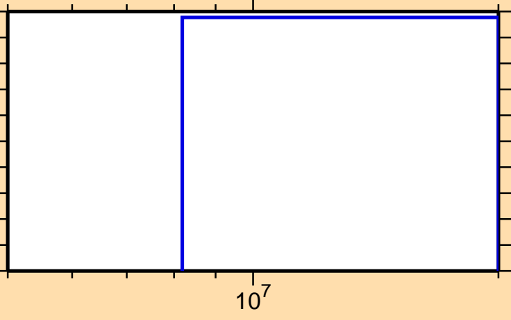
\sigma vs. E for ^{246}\text{Es}(n,3n)
