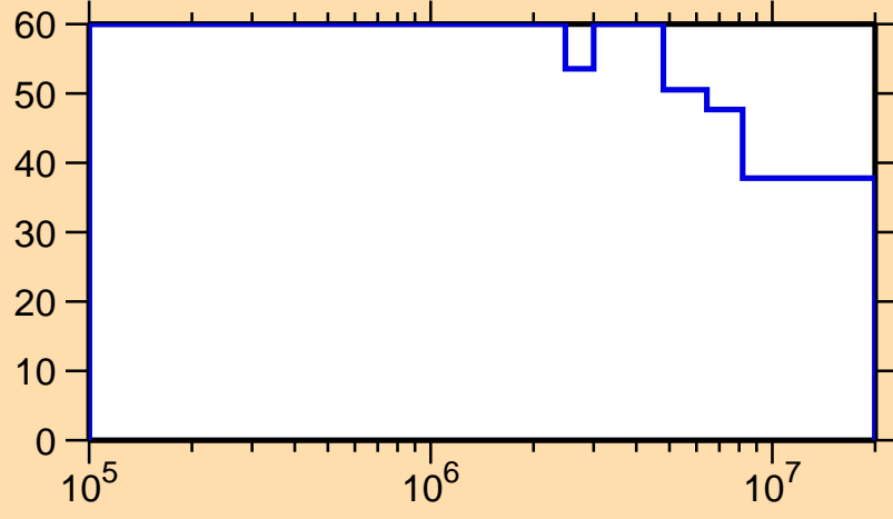
\Delta\sigma/\sigma vs. E for ^{246}\text{Es}(n,n_1)
