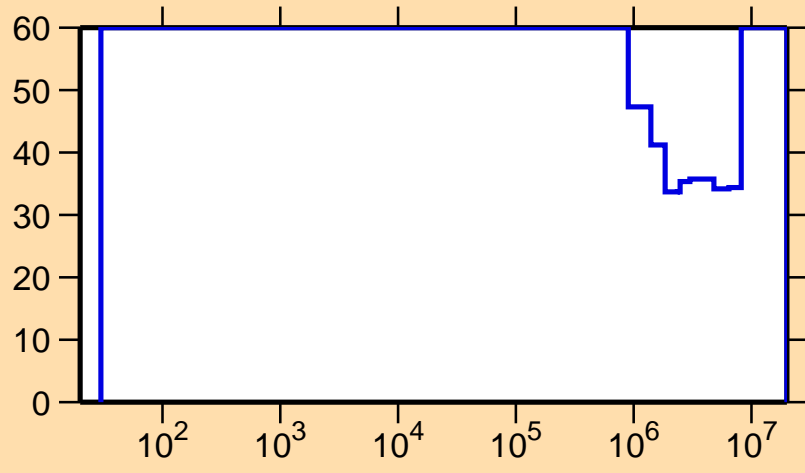
\Delta\sigma/\sigma vs. E for ^{246}\text{Es}(n,p)
