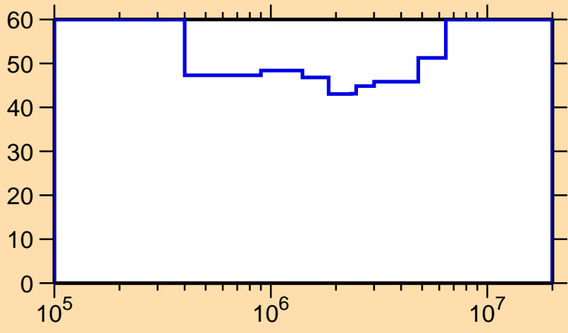
\Delta\sigma/\sigma vs. E for ^{246}\text{Es}(n,n\text{cont.})
