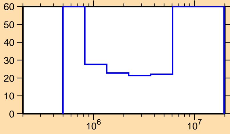
\Delta\sigma/\sigma vs. E for ^{247}\text{Es}(n,n\text{cont.})
