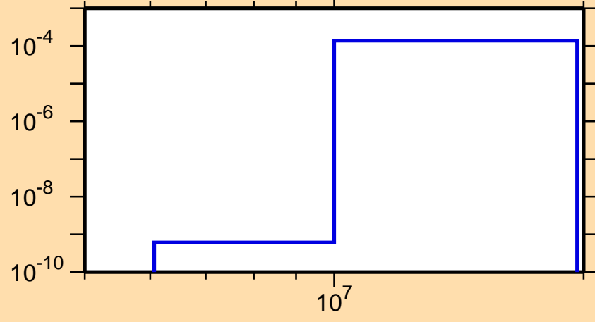
\sigma vs. E for ^{247}\text{Es} (mt 45)
