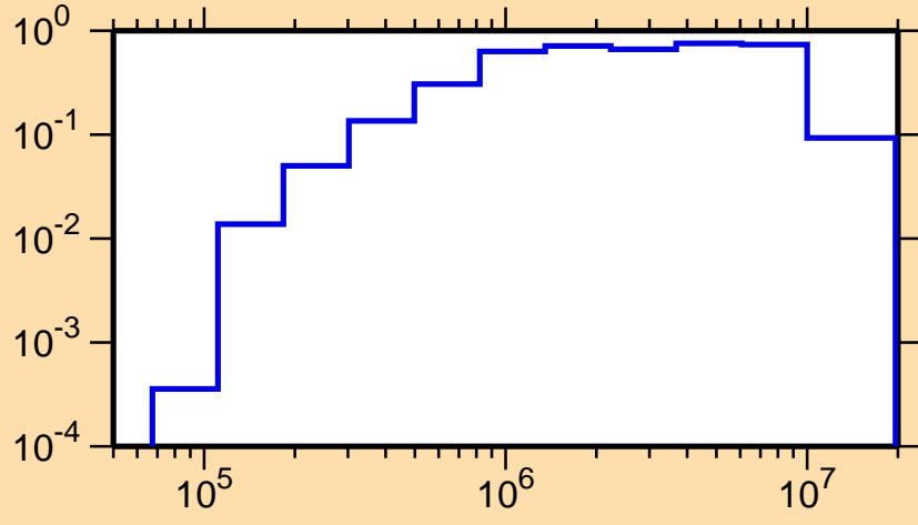
\sigma vs. E for ^{248}\text{Es}(n,n\alpha)
