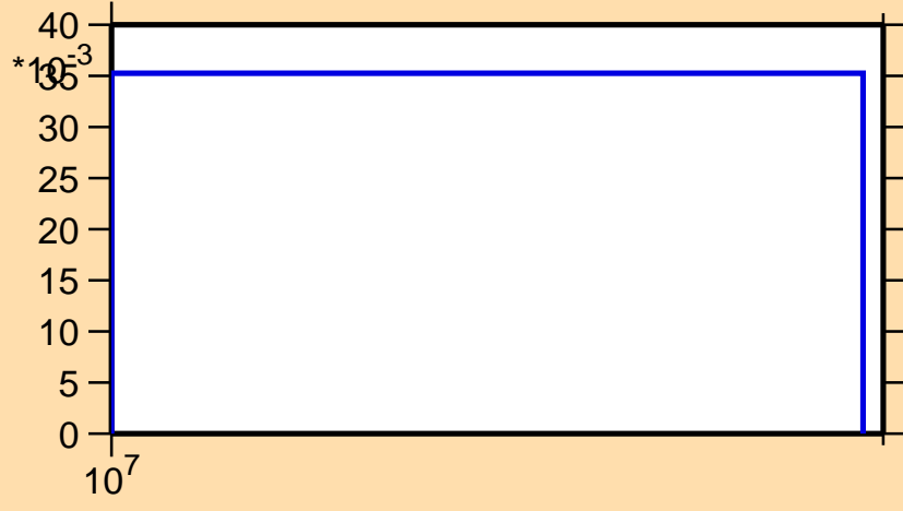
\sigma vs. E for ^{248}\text{Es}(n,3n\alpha)
