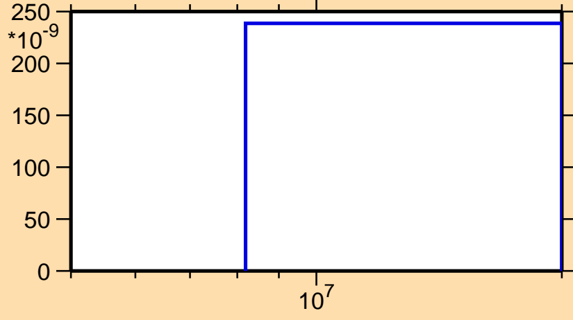
\sigma vs. E for ^{248}\text{Es}(n,nd)
