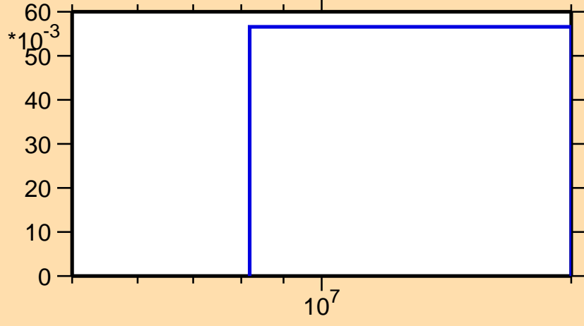
\sigma vs. E for ^{248}\text{Es}(n,3n)
