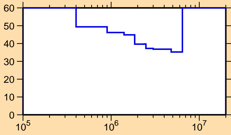
\Delta\sigma/\sigma vs. E for ^{248}\text{Es}(n,n\text{cont.})
