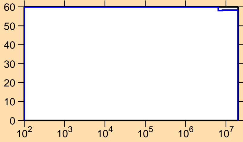
\Delta\sigma/\sigma vs. E for ^{248}\text{Es}(n,p)
