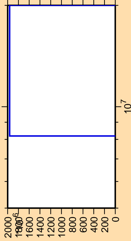
\Delta\sigma/\sigma vs. E for ^{248}\text{Es} (mt 42)
