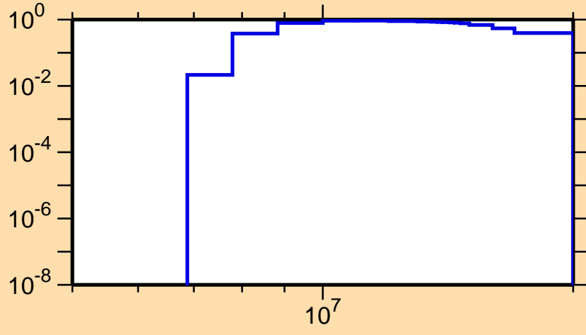
\sigma vs. E for ^{249}\text{Es}(n,2n\alpha)
