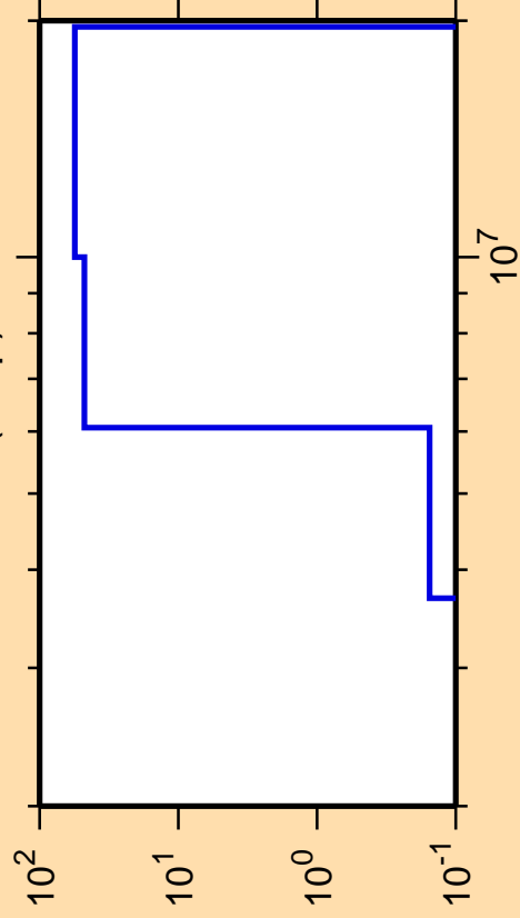
\Delta\sigma/\sigma vs. E for ^{249}\text{Es}(n,np)
