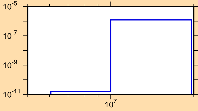
\sigma vs. E for ^{249}\text{Es}(\text{mt117})
