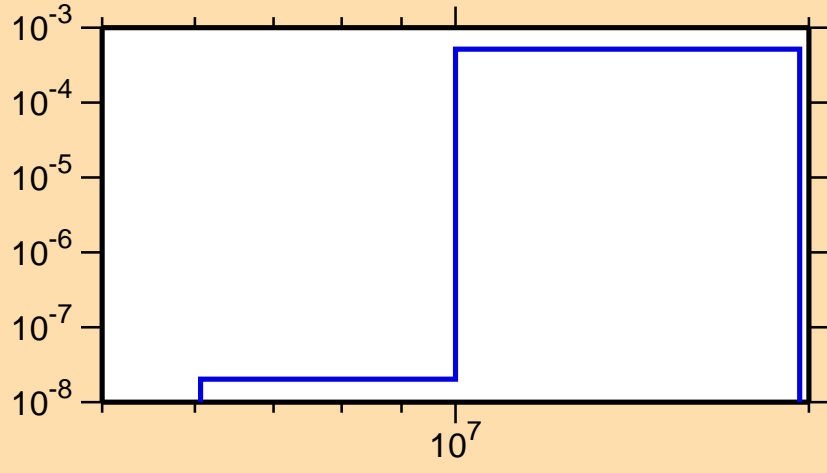
\sigma vs. E for ^{249}\text{Es}(n,d)
