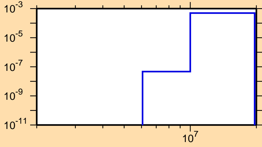
\sigma vs. E for ^{249}\text{Es}(n,np)
