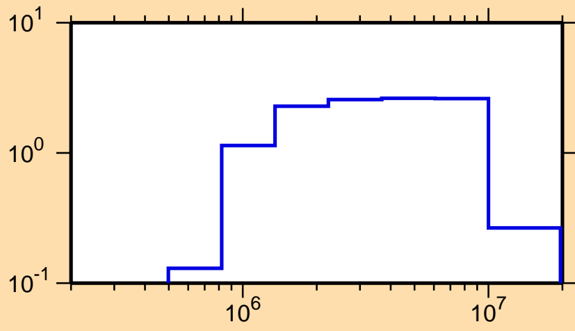
\sigma vs. E for ^{249}\text{Es}(n,n\text{cont.})
