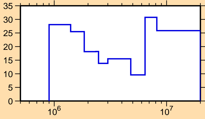
\Delta\sigma/\sigma vs. E for ^{249}\text{Es}(n,n\text{cont.})
