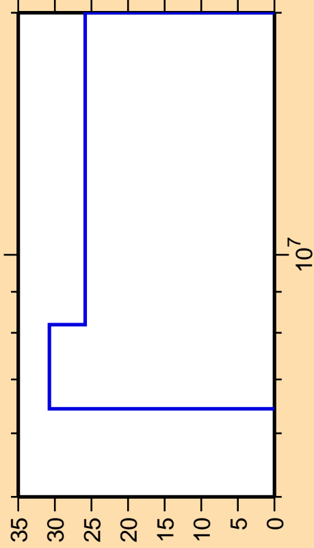
\Delta\sigma/\sigma vs. E for ^{249}\text{Es}(n,n\text{cont.})
