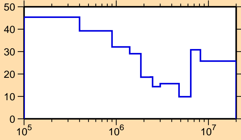
\Delta\sigma/\sigma vs. E for ^{249}\text{Es}(n,\text{inel.})
