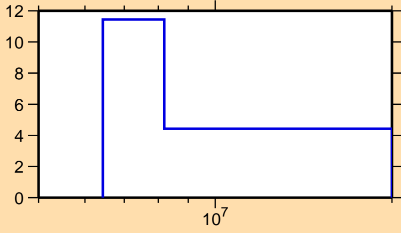
\Delta\sigma/\sigma vs. E for ^{249}\text{Es}(n,\text{tot.})
