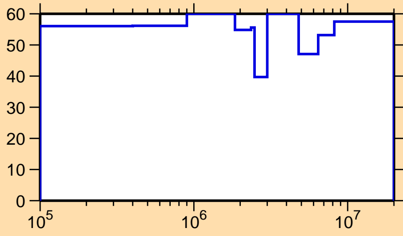
\Delta\sigma/\sigma vs. E for ^{249}\text{Es}(n,n_1)
