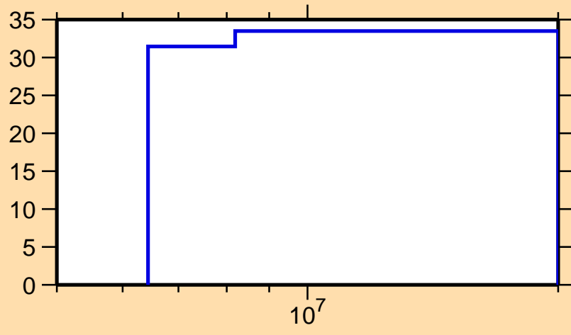
\Delta\sigma/\sigma vs. E for ^{249}\text{Es}(n,2n)
