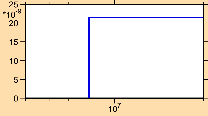
\sigma vs. E for ^{249}\text{Es}(n,nt)
