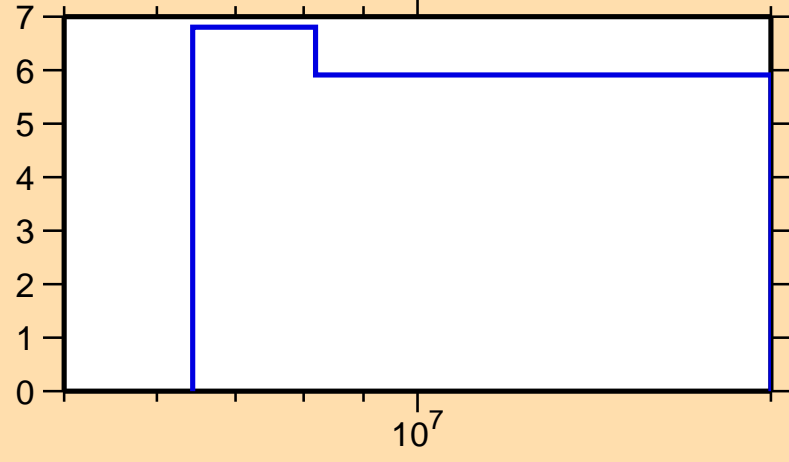
\Delta\sigma/\sigma vs. E for ^{249}\text{Es}(n,\text{nonel.})
