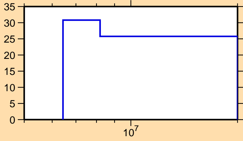
\Delta\sigma/\sigma vs. E for ^{249}\text{Es}(n,\text{inel.})
