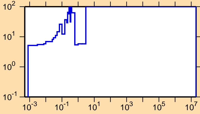
\Delta\sigma/\sigma vs. E for ^{249}\text{Es}(n,f)
