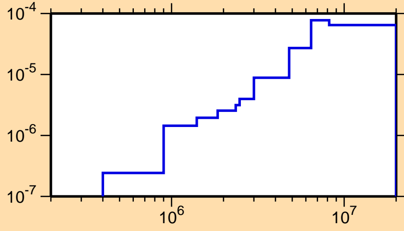
\sigma vs. E for ^{249}\text{Es}(n,n\alpha)
