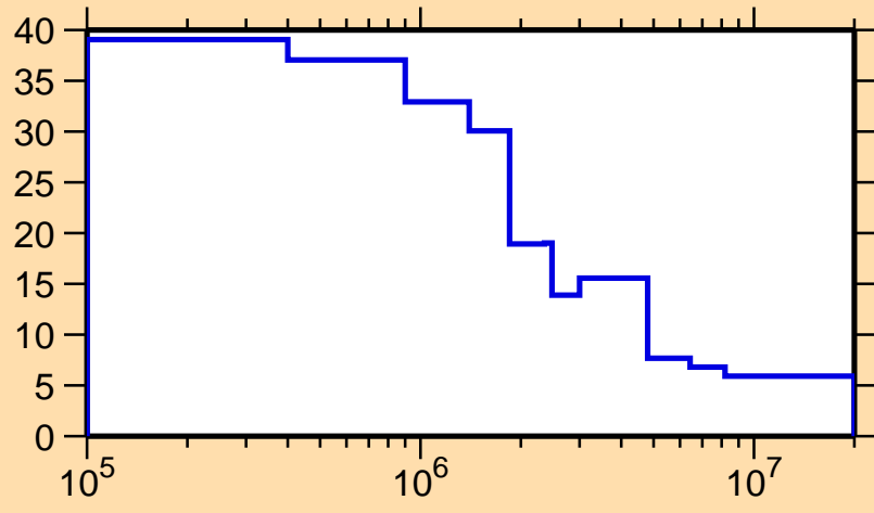
\Delta\sigma/\sigma vs. E for ^{249}\text{Es}(n,\text{nonel.})
