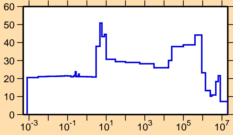
\Delta\sigma/\sigma vs. E for ^{249}\text{Es}(n,el.)
