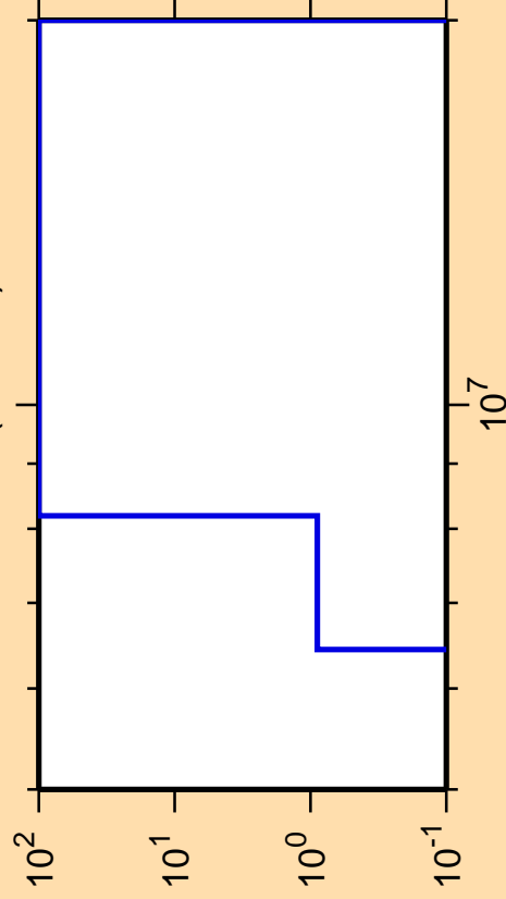
\Delta\sigma/\sigma vs. E for ^{249}\text{Es}(\text{mt117})
