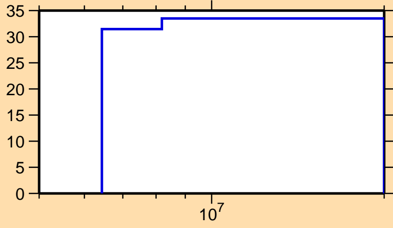
\Delta\sigma/\sigma vs. E for ^{249}\text{Es}(n,2n)
