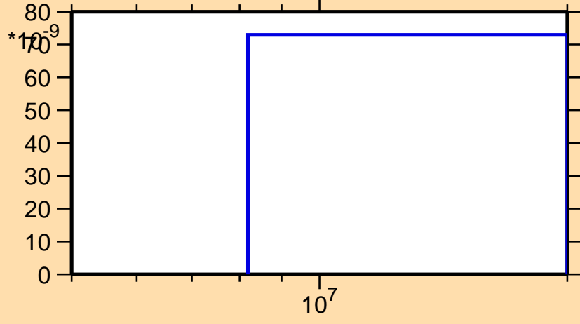
\sigma vs. E for ^{249}\text{Es}(n,2np)
