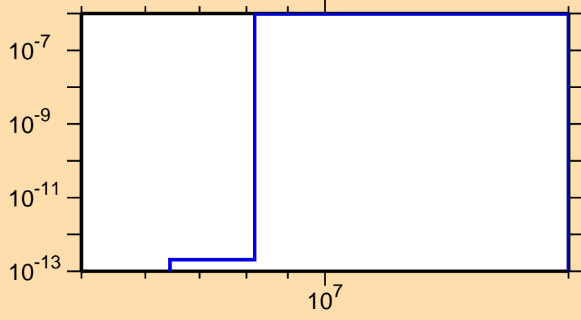
\sigma vs. E for ^{249}\text{Es}(\text{mt117})
