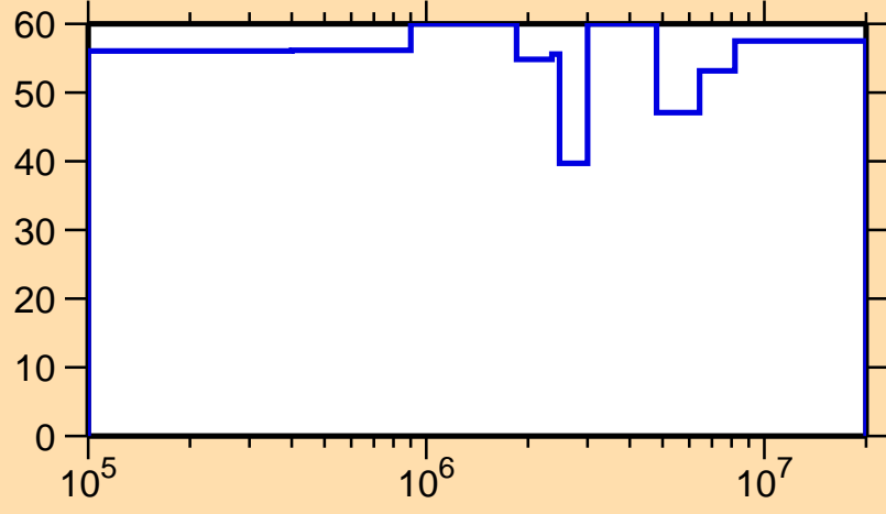
\Delta\sigma/\sigma vs. E for ^{249}\text{Es}(n,n_1)
