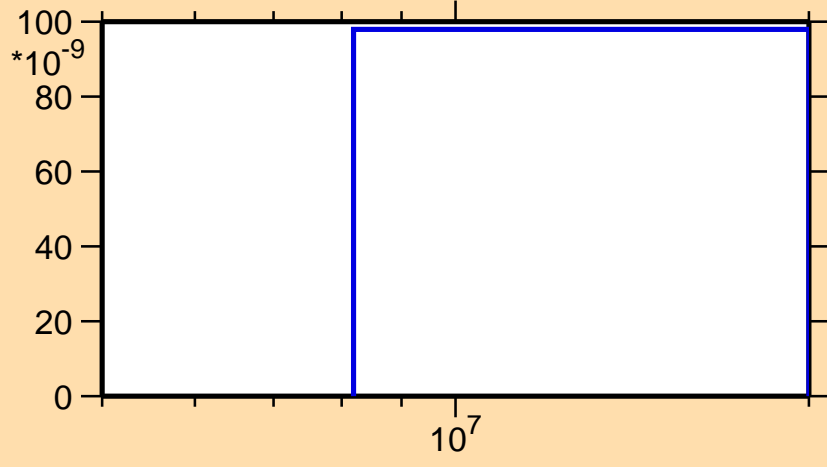
\sigma vs. E for ^{249}\text{Es}(n,nd)
