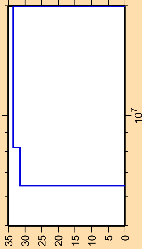
\Delta\sigma/\sigma vs. E for ^{249}\text{Es}(n,2n)
