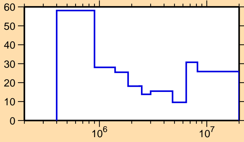
\Delta\sigma/\sigma vs. E for ^{249}\text{Es}(n,n\text{cont.})
