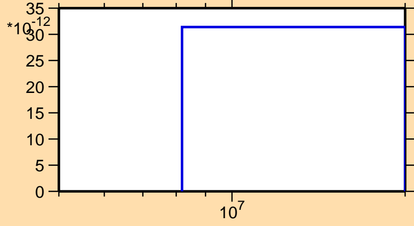
\sigma vs. E for ^{249}\text{Es}(n,\text{He3})
