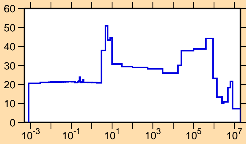
\Delta\sigma/\sigma vs. E for ^{249}\text{Es}(n,\text{el.})
