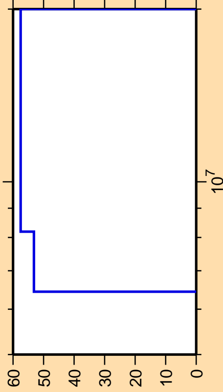
\Delta\sigma/\sigma vs. E for ^{249}\text{Es}(n,n_1)
