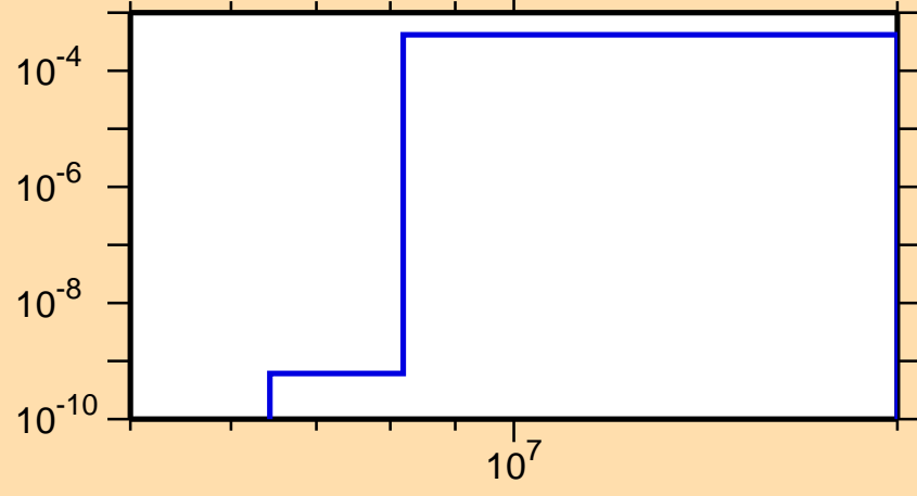
\sigma vs. E for ^{249}\text{Es}(n,d)
