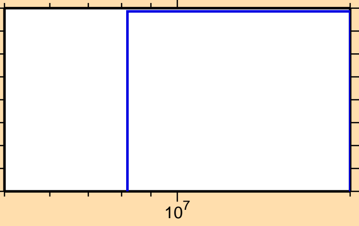
\sigma vs. E for ^{249}\text{Es}(n,3n)
