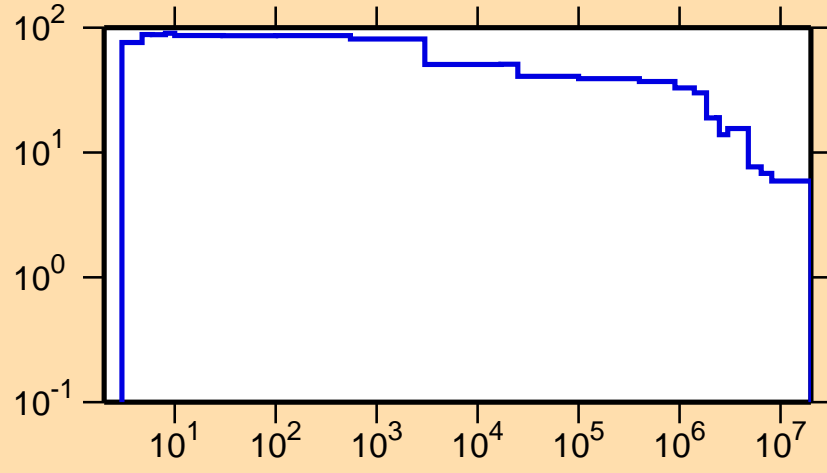
\Delta\sigma/\sigma vs. E for ^{249}\text{Es}(n,\text{nonel.})
