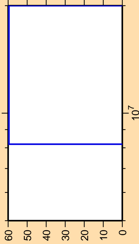
\Delta\sigma/\sigma vs. E for ^{249}\text{Es}(n,nd)
