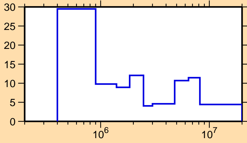
\Delta\sigma/\sigma vs. E for ^{249}\text{Es}(n, \text{tot.})
