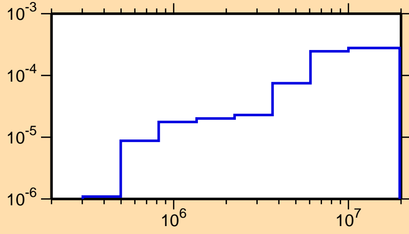
\sigma vs. E for ^{250}\text{Es}(n,n\alpha)
