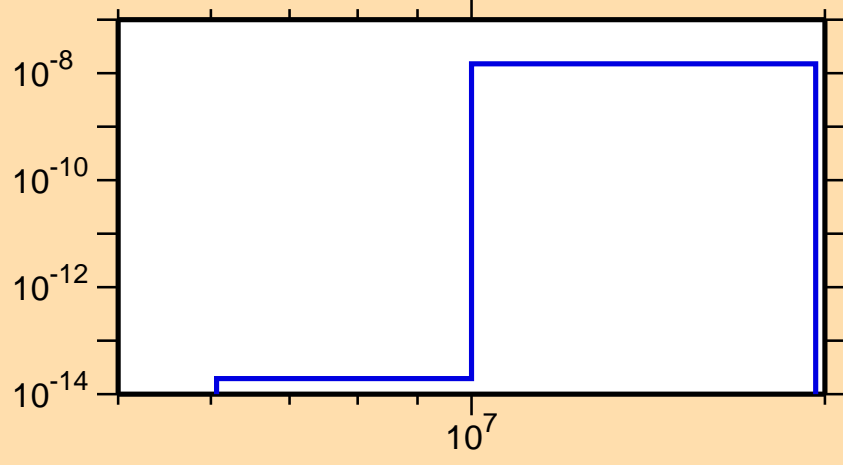
\sigma vs. E for ^{250}\text{Es}(\text{mt117})
