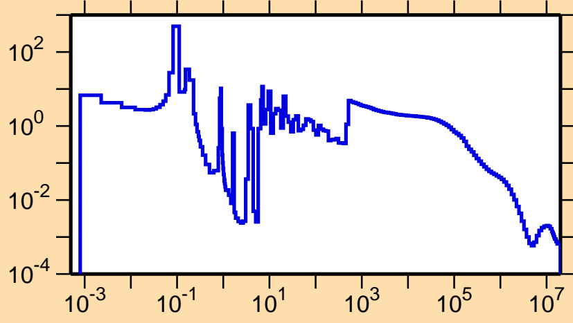
\sigma vs. E for ^{250}\text{Es}(n,\gamma)
