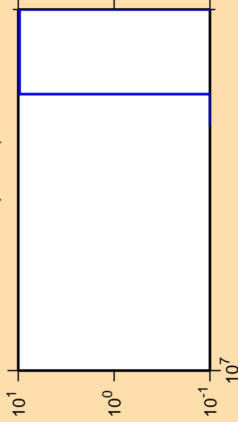
\Delta\sigma/\sigma vs. E for ^{250}\text{Es} (mt 11)
