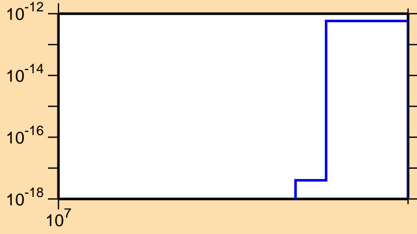
\sigma vs. E for ^{250}\text{Es} (mt 42)
