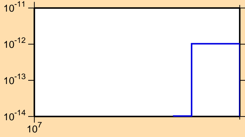
\sigma vs. E for ^{250}\text{Es} (mt 34)
