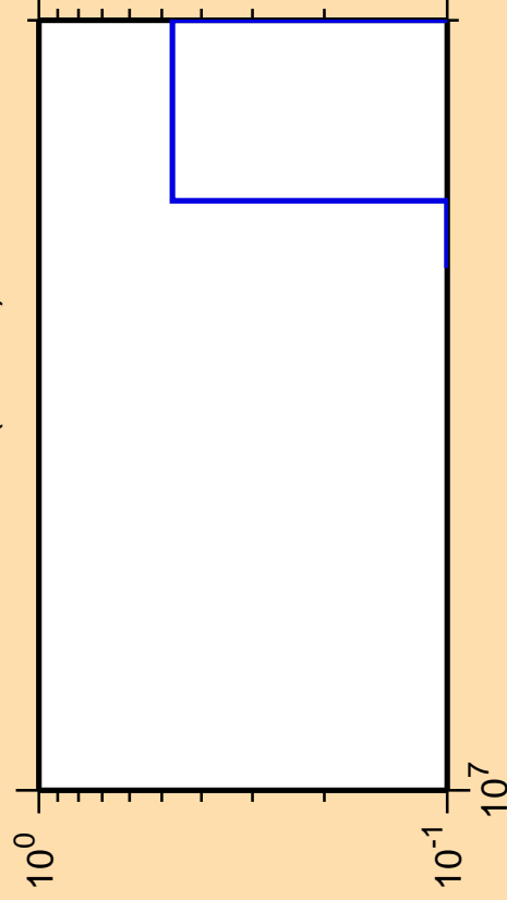
\Delta\sigma/\sigma vs. E for ^{250}\text{Es} (mt 42)
