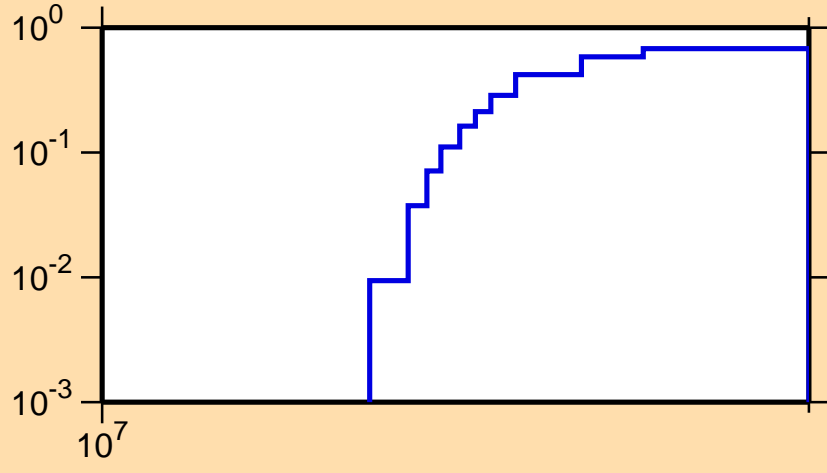
\sigma vs. E for ^{250}\text{Es}(n,3n\alpha)
