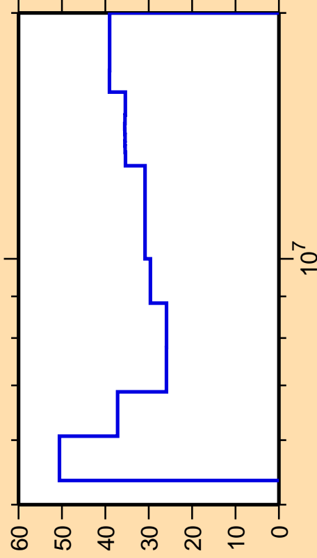
\Delta\sigma/\sigma vs. E for ^{250}\text{Es}(n,2n)
