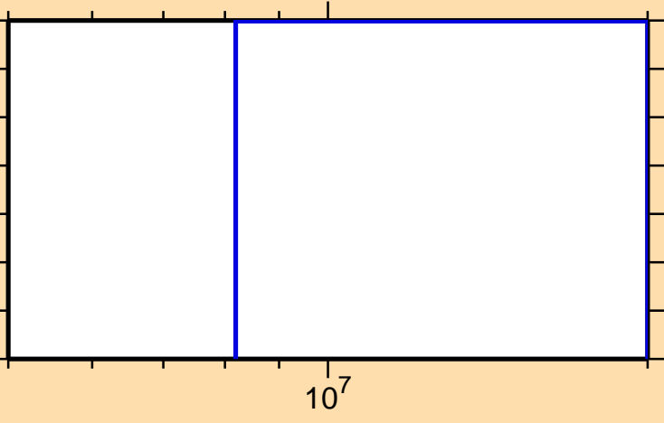
\sigma vs. E for ^{250}\text{Es}(n,3n)
