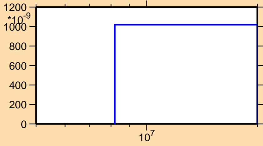
\sigma vs. E for ^{250}\text{Es}(n,nd)
