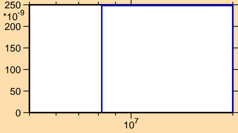
\sigma vs. E for ^{250}\text{Es}(n,nt)
