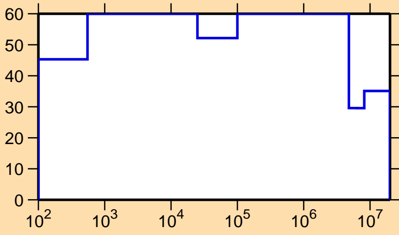
\Delta\sigma/\sigma vs. E for ^{250}\text{Es}(n,p)
