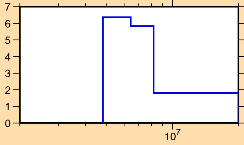
\Delta\sigma/\sigma vs. E for ^{250}\text{Es}(n,\text{tot.})
