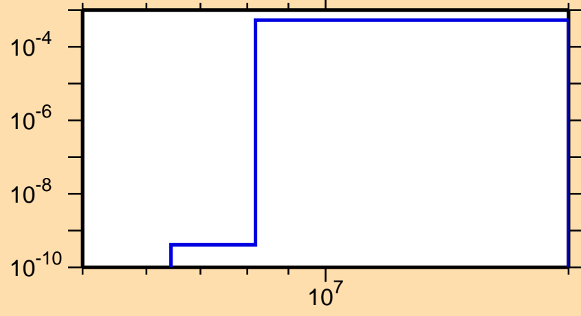
\sigma vs. E for ^{250}\text{Es}(n,d)
