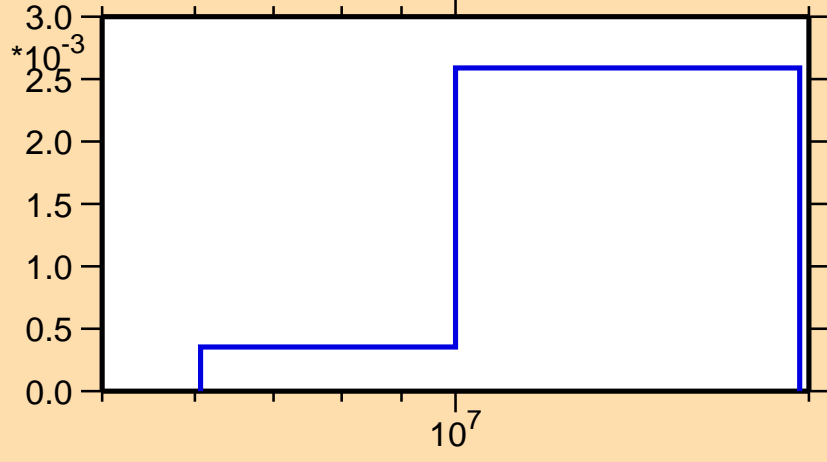
\sigma vs. E for ^{251}\text{Es}(n,2n\alpha)
