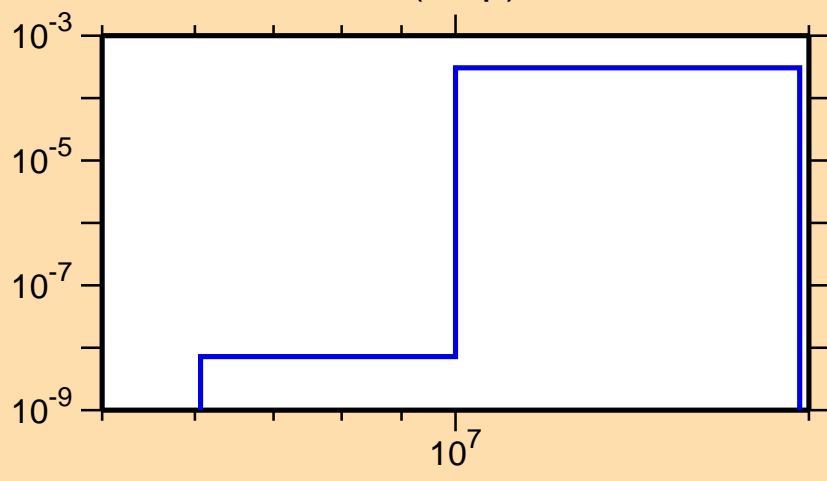
\sigma vs. E for ^{251}\text{Es}(n,np)
