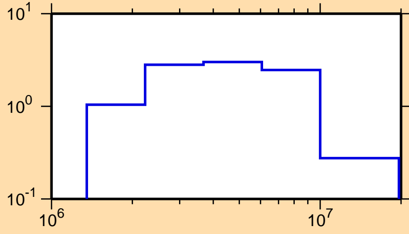
\sigma vs. E for ^{251}\text{Es}(n,n\text{cont.})
