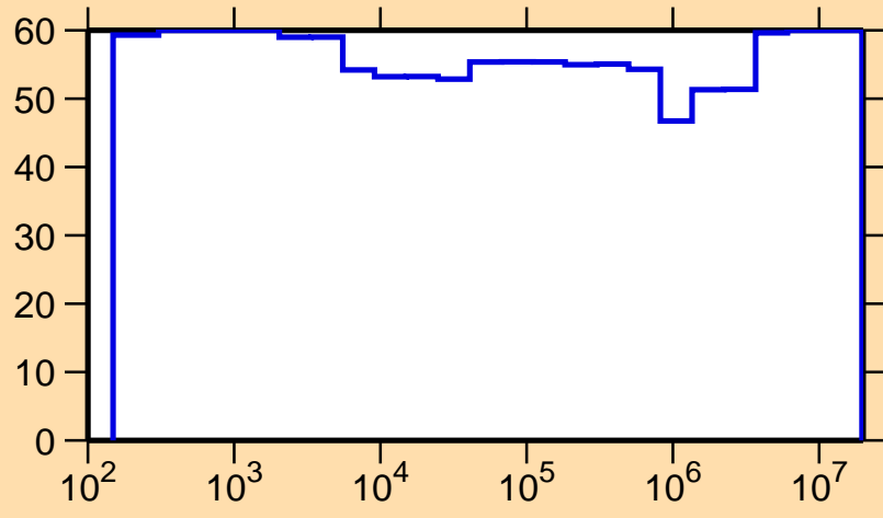
\Delta\sigma/\sigma vs. E for ^{251}\text{Es}(n,\gamma)
