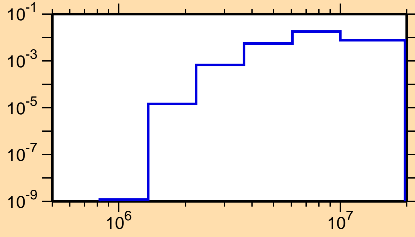
\sigma vs. E for ^{251}\text{Es}(n,n\alpha)
