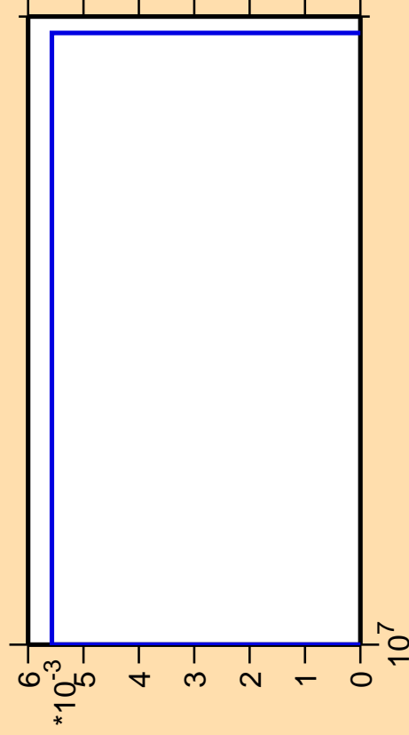
\Delta\sigma/\sigma vs. E for ^{251}\text{Es} (mt 11)
