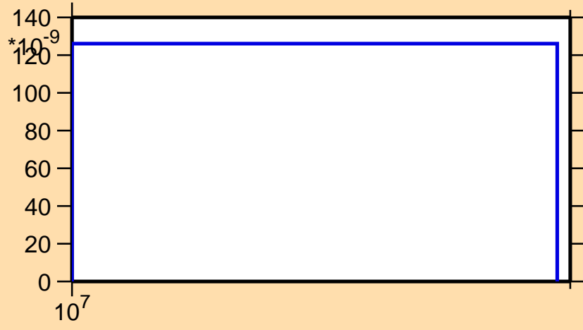
\sigma vs. E for ^{251}\text{Es}(n,nt)
