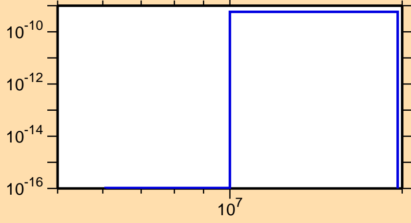
\sigma vs. E for ^{251}\text{Es}(\text{mt } 45)
