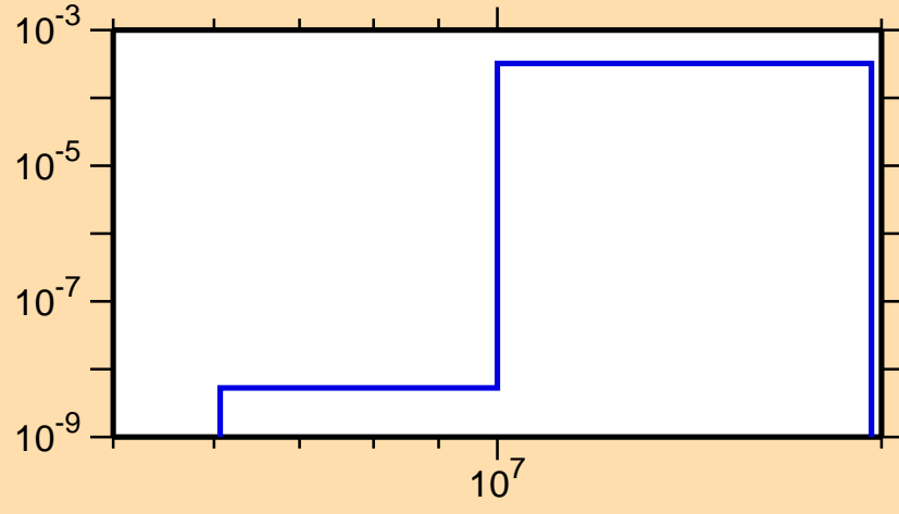
\sigma vs. E for ^{251}\text{Es}(n,d)
