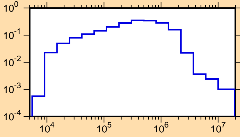
\sigma vs. E for ^{251}\text{Es}(n,n_1)
