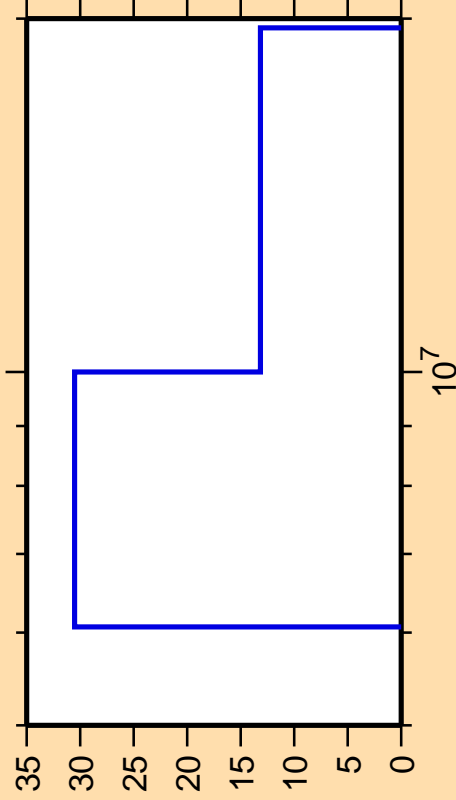
\Delta\sigma/\sigma vs. E for ^{251}\text{Es}(n,d)
