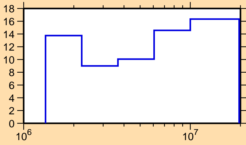
\Delta\sigma/\sigma vs. E for ^{251}\text{Es}(n,\text{inel.})
