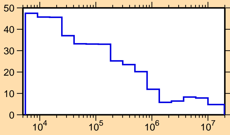
\Delta\sigma/\sigma vs. E for ^{251}\text{Es}(n,\text{el.})
