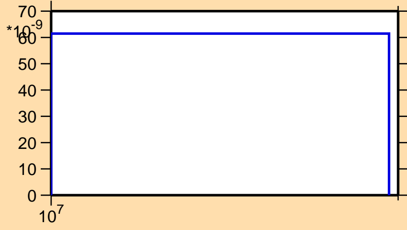
\sigma vs. E for ^{251}\text{Es}(n,nd)
