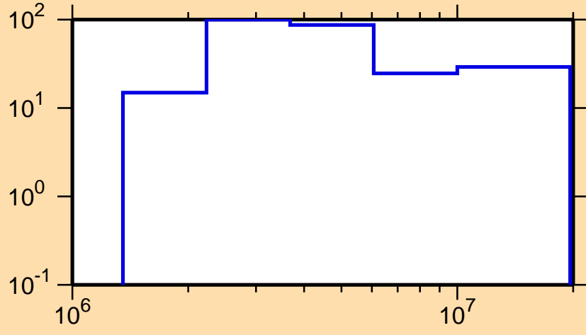
\Delta\sigma/\sigma vs. E for ^{251}\text{Es}(n,p)
