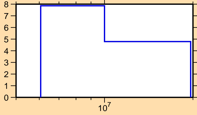
\Delta\sigma/\sigma vs. E for ^{251}\text{Es}(n,\text{el.})
