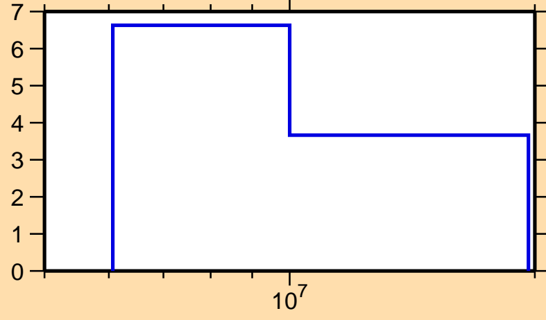
\Delta\sigma/\sigma vs. E for ^{251}\text{Es}(n,\text{tot.})
