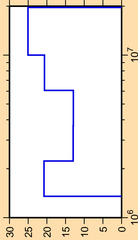
\Delta\sigma/\sigma vs. E for ^{251}\text{Es}(n,n\text{cont.})
