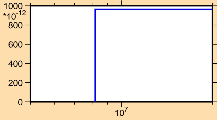
\sigma vs. E for ^{251}\text{Es}(\text{mt117})
