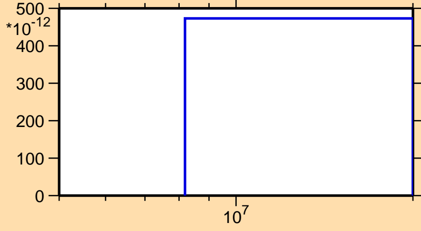
\sigma vs. E for ^{251}\text{Es} (mt 45)
