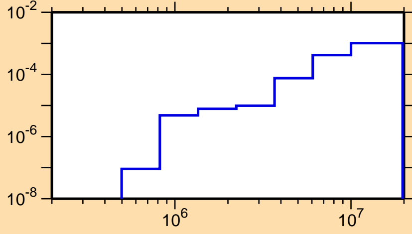
\sigma vs. E for ^{253}\text{Es}(n,n\alpha)
