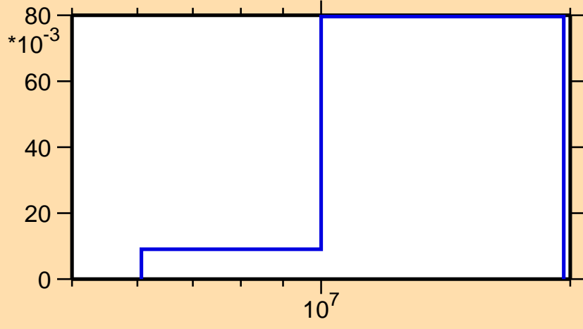
\sigma vs. E for ^{253}\text{Es}(n,2n\alpha)
