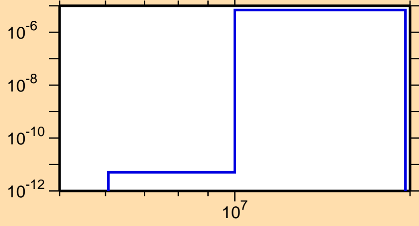
\sigma vs. E for ^{253}\text{Es}(\text{mt117})
