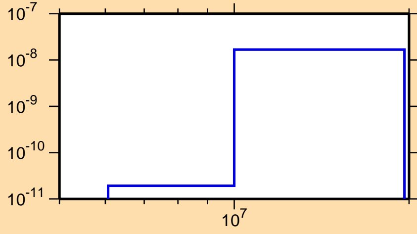
\sigma vs. E for ^{253}\text{Es}(n,p\alpha)
