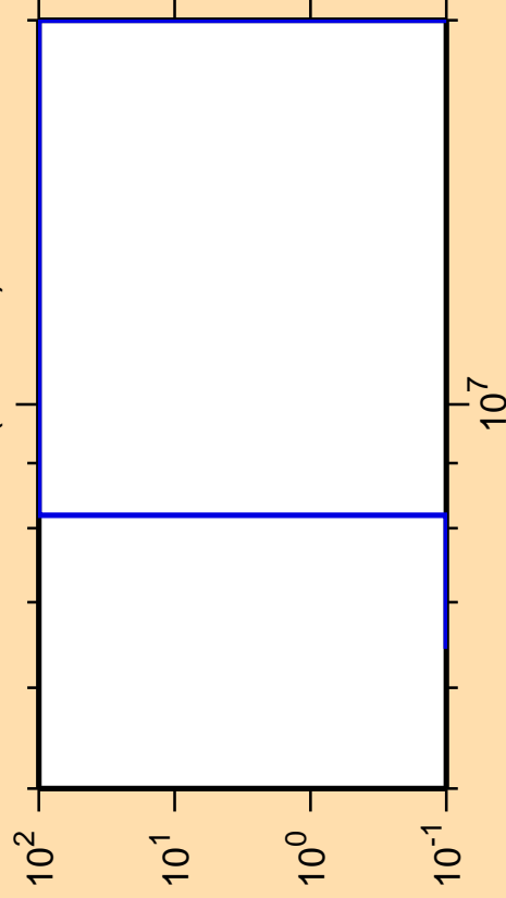
\Delta\sigma/\sigma vs. E for ^{253}\text{Es}(\text{mt117})
