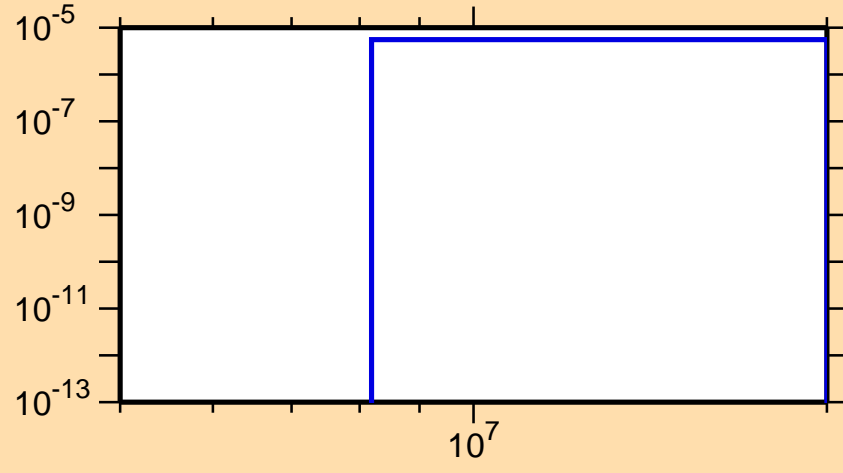
\sigma vs. E for ^{253}\text{Es}(\text{mt117})
