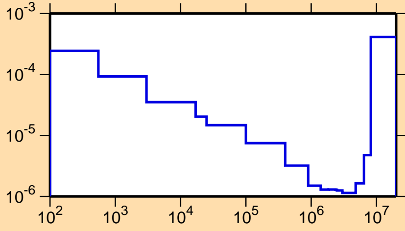
\sigma vs. E for ^{253}\text{Es}(n,\alpha)
