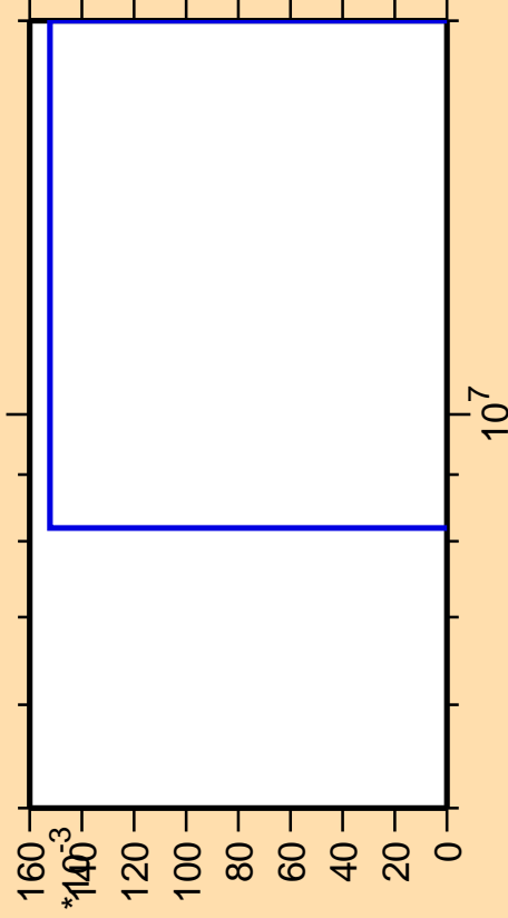
\Delta\sigma/\sigma vs. E for ^{253}\text{Es}(n,\text{He3})
