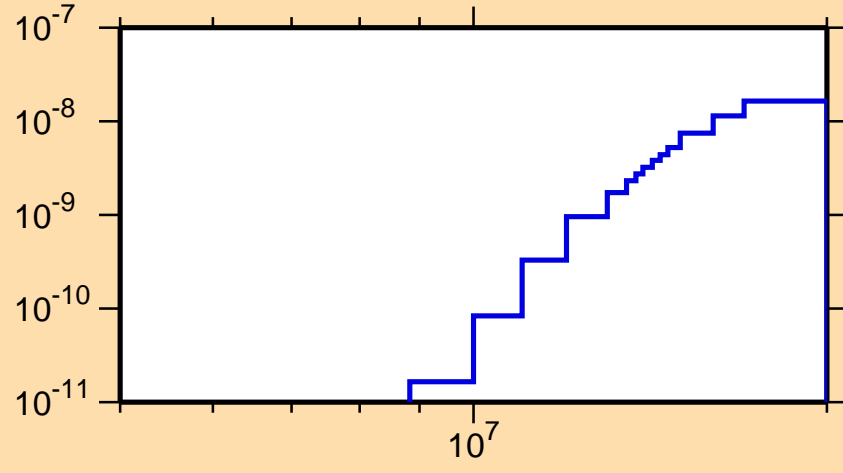
\sigma vs. E for ^{254}\text{Es}(n,p\alpha)
