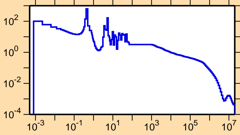
\sigma vs. E for ^{254}\text{Es}(n,\gamma)
