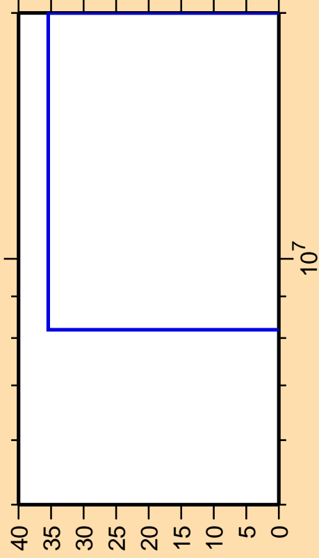
\Delta\sigma/\sigma vs. E for ^{254}\text{Es}(n,p\alpha)
