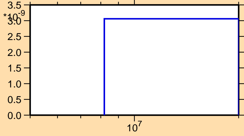
\sigma vs. E for ^{254}\text{Es}(n,p\alpha)
