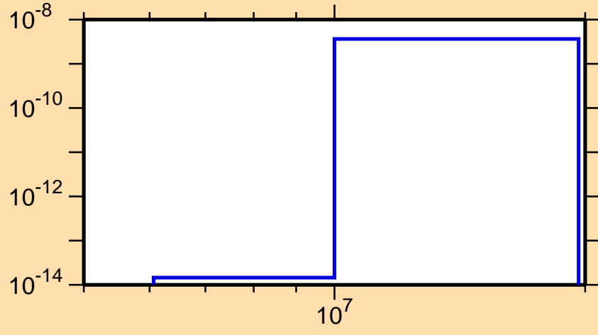
\sigma vs. E for ^{254}\text{Es}(\text{mt117})
