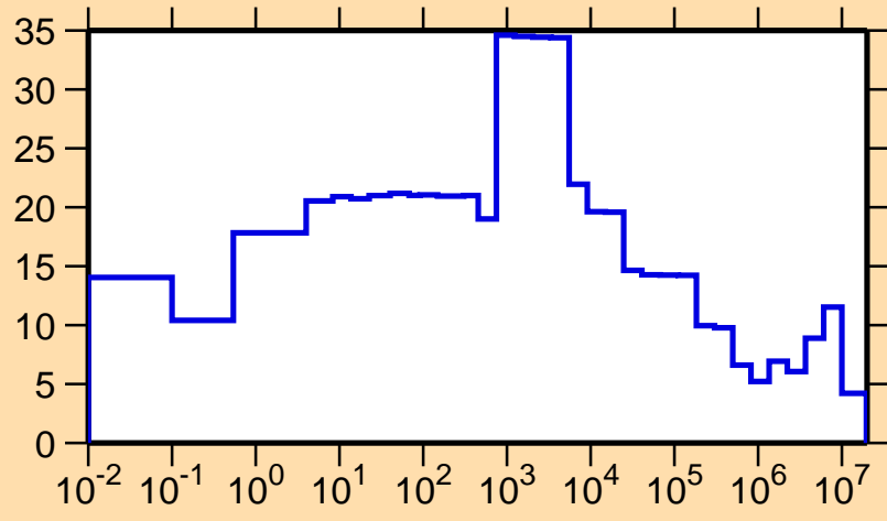
\Delta\sigma/\sigma vs. E for ^{254}\text{Es}(n,el.)
