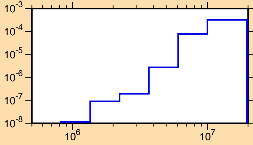
\sigma vs. E for ^{256}\text{Es}(n,n_3)
