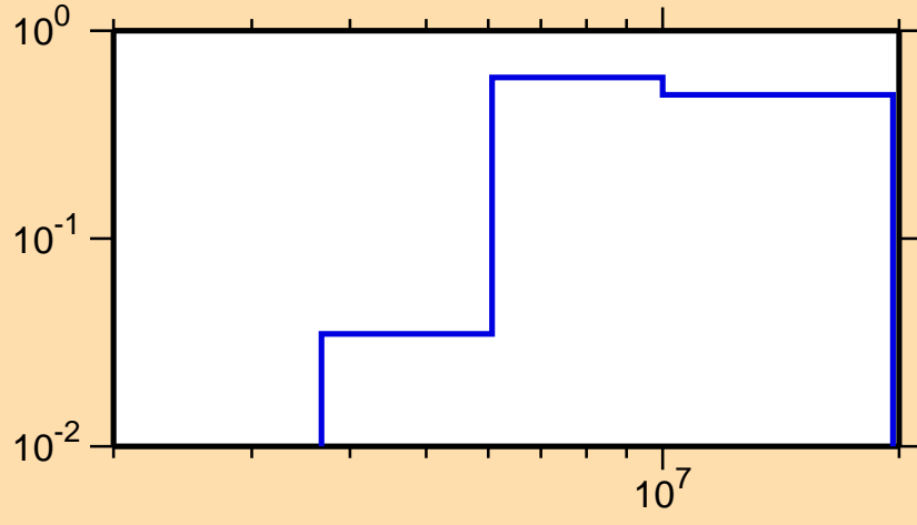
\sigma vs. E for ^{256}\text{Es}(n,2n)
