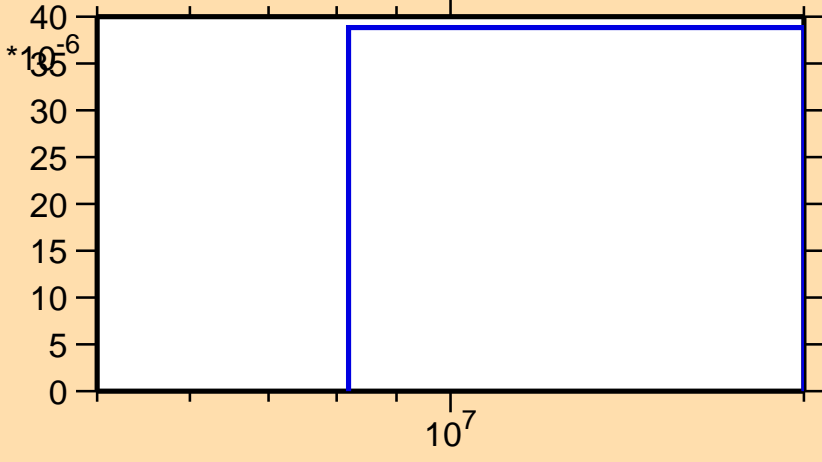
\sigma vs. E for ^{256}\text{Es}(n,np)
