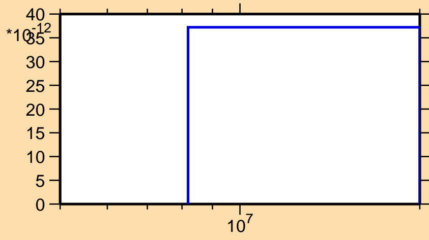
\sigma vs. E for ^{256}\text{Es}(n,p\alpha)
