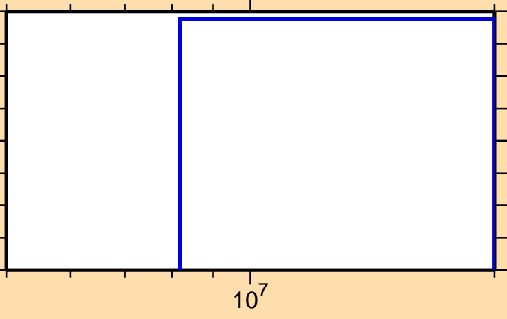
\sigma vs. E for ^{256}\text{Es}(n,np)
