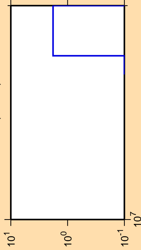
\Delta\sigma/\sigma vs. E for ^{257}\text{Es} (mt 42)
