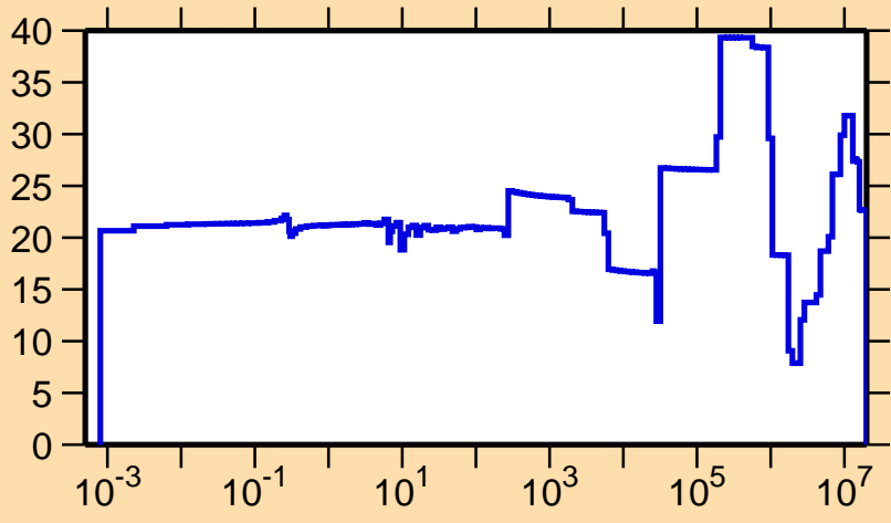
\Delta\sigma/\sigma vs. E for ^{257}\text{Es}(n,el.)
