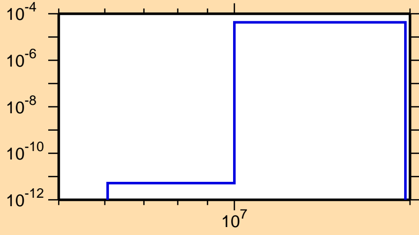
\sigma vs. E for ^{257}\text{Es}(n,np)
