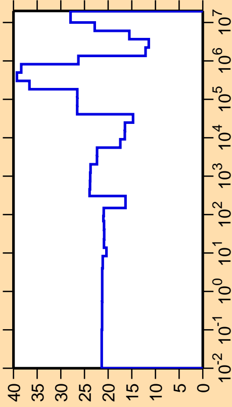
\Delta\sigma/\sigma vs. E for ^{257}\text{Es}(n,\text{el.})
