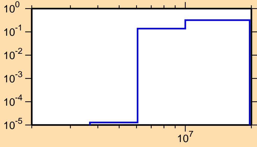
\sigma vs. E for ^{257}\text{Es}(n,2n)
