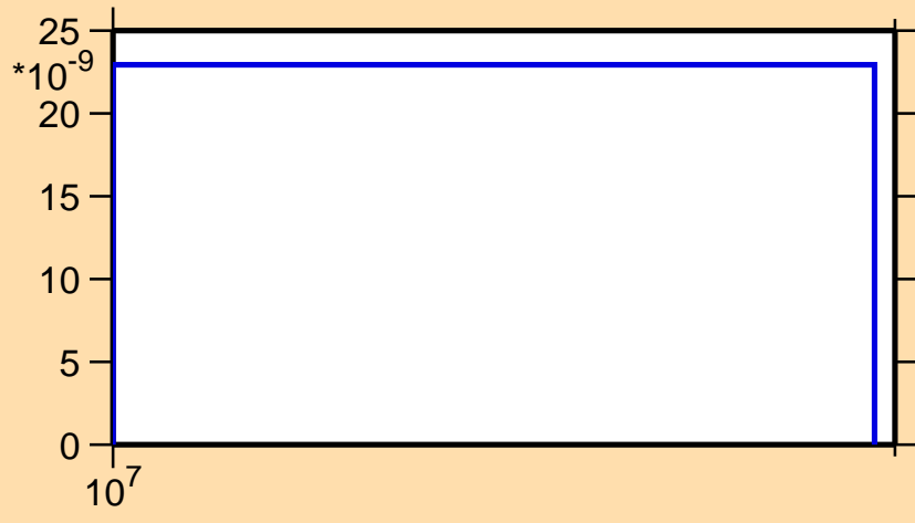
\sigma vs. E for ^{257}\text{Es}(n,nd)
