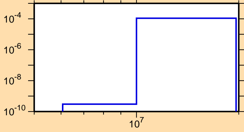
\sigma vs. E for ^{257}\text{Es}(n,d)
