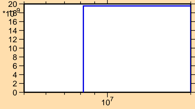
\sigma vs. E for ^{257}\text{Es}(n,nd)
