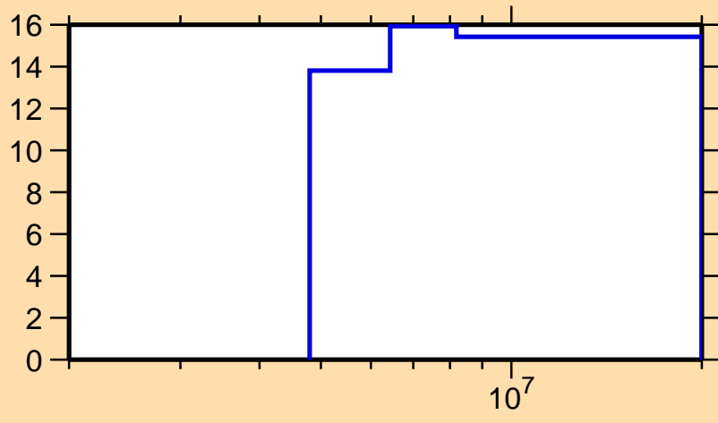
Δσ/σ vs. E for ^{257}\text{Es}(n,\text{tot.})
