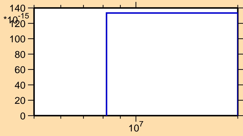
\sigma vs. E for ^{257}\text{Es} (mt 11)
