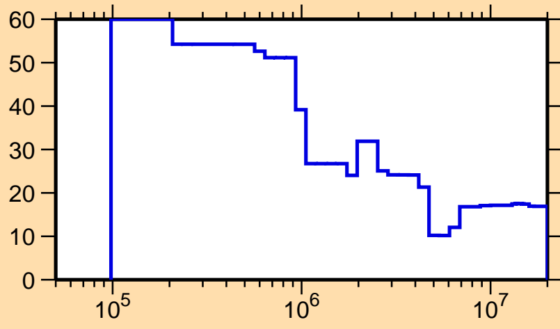
\Delta\sigma/\sigma vs. E for ^{258}\text{Es}(n,\text{nonel.})
