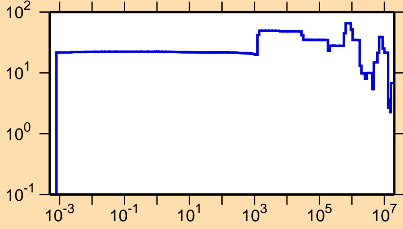
\Delta\sigma/\sigma vs. E for ^{258}\text{Es}(n,el.)
