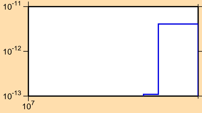
\sigma vs. E for ^{258}\text{Es}(n,\text{He3})
