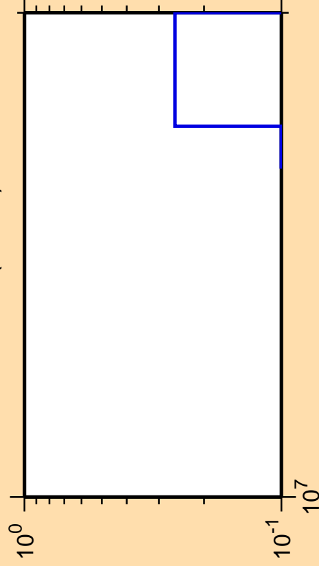
\Delta\sigma/\sigma vs. E for ^{258}\text{Es} (mt 42)
