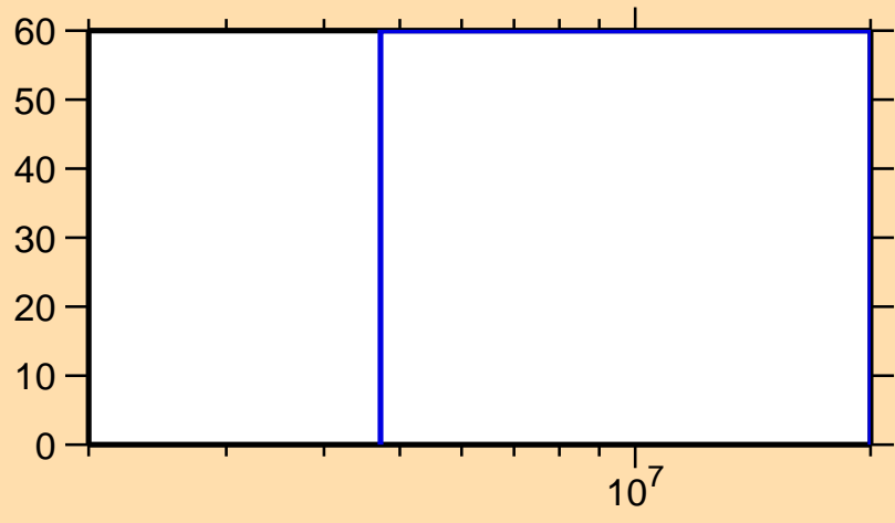
\Delta\sigma/\sigma vs. E for ^{258}\text{Es}(n,2n)
