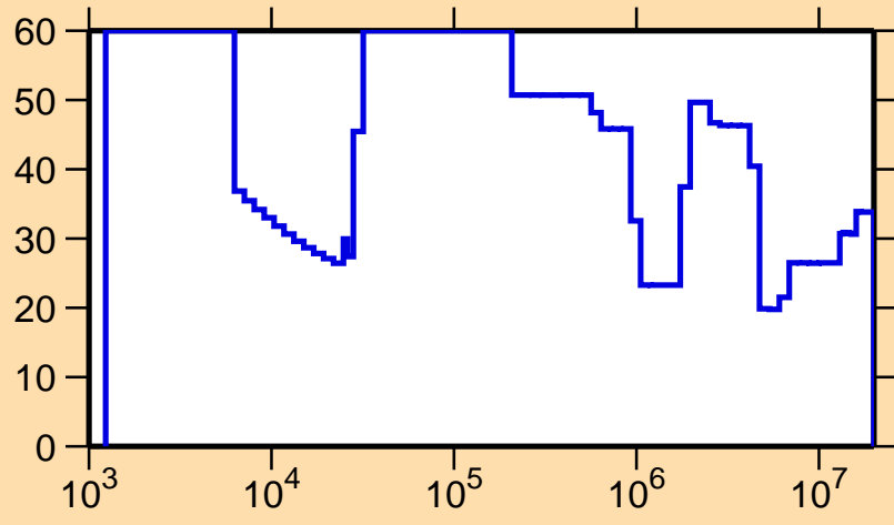
\Delta\sigma/\sigma vs. E for ^{258}\text{Es}(n,f)
