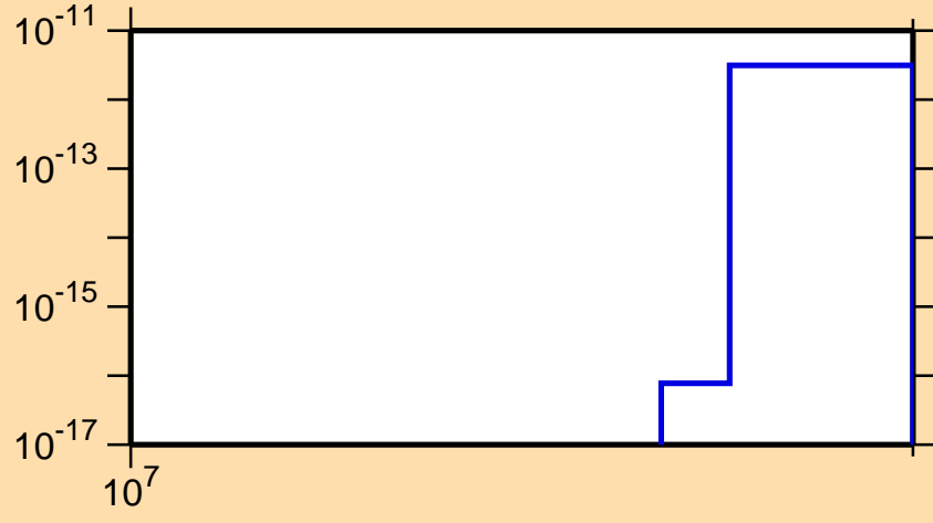
\sigma vs. E for ^{258}\text{Es} (mt 11)
