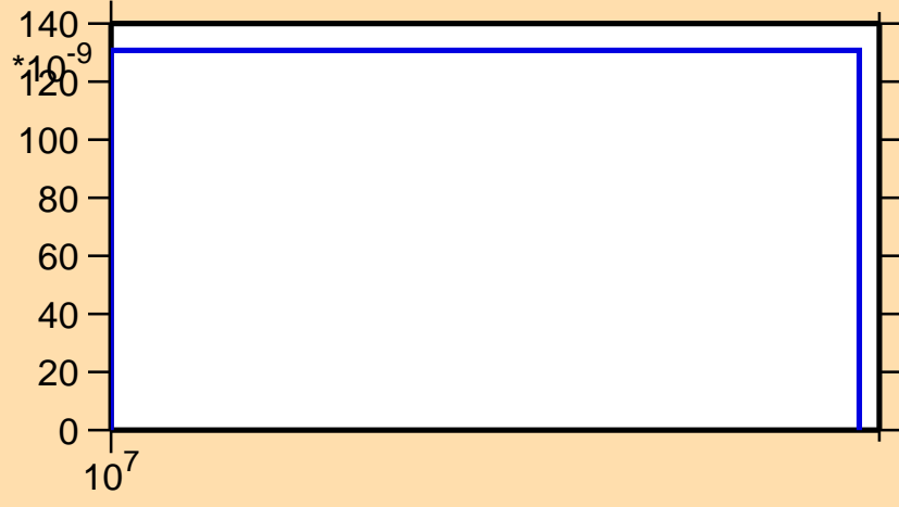
\sigma vs. E for ^{258}\text{Es}(n,nt)
