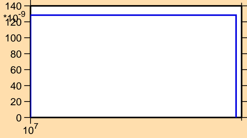
\sigma vs. E for ^{258}\text{Es}(n,nd)
