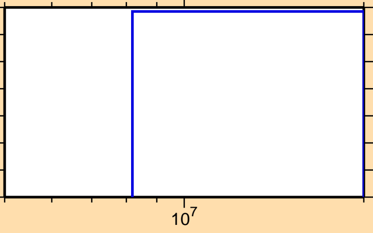
\sigma vs. E for ^{258}\text{Es}(n,2np)
