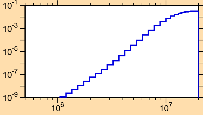
\sigma vs. E for ^{135}\text{Eu}(n,d)
