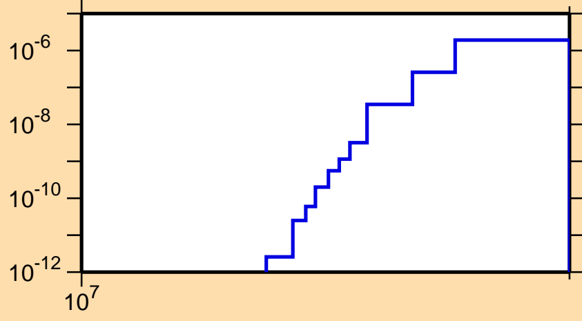
\sigma vs. E for ^{135}\text{Eu}(n,\text{nd})
