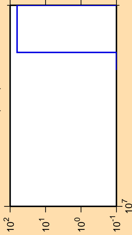
\Delta\sigma/\sigma vs. E for ^{135}\text{Eu}(n,nt)
