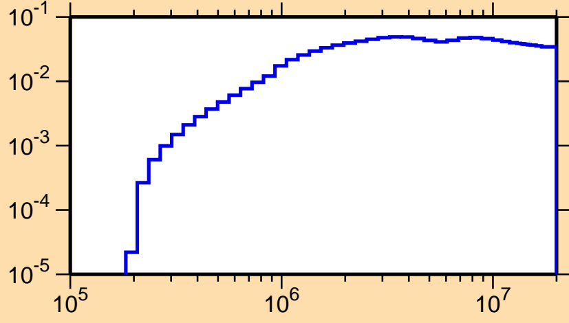
\sigma vs. E for ^{135}\text{Eu}(n,n\text{cont.})
