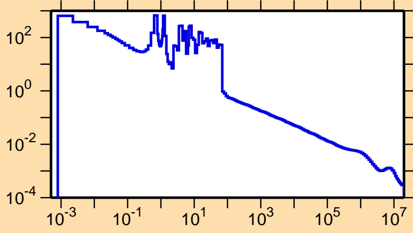
\sigma vs. E for ^{135}\text{Eu}(n,\gamma)
