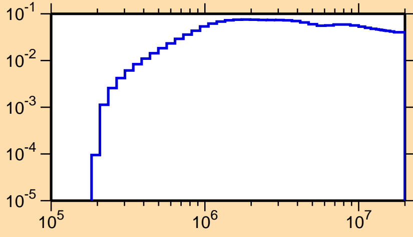
\sigma vs. E for ^{135}\text{Eu}(n,\text{inel.})
