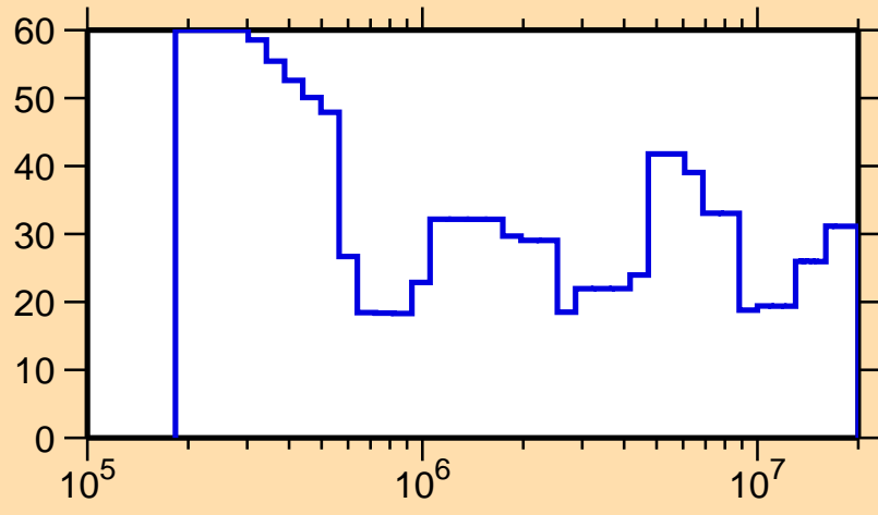
\Delta\sigma/\sigma vs. E for ^{135}\text{Eu}(n,\text{el.})
