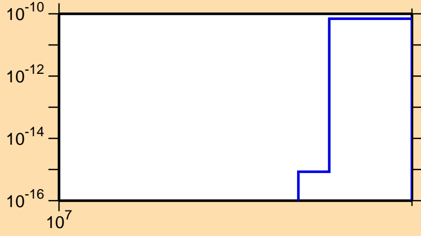
\sigma vs. E for ^{135}\text{Eu}(n,nt)
