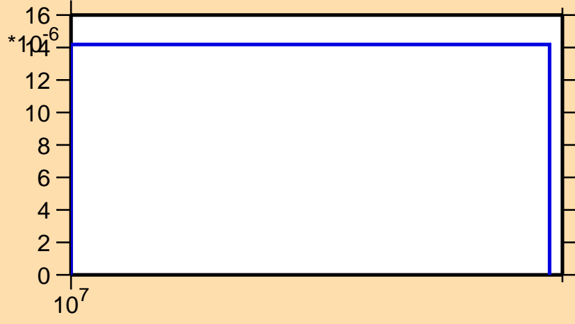
\sigma vs. E for ^{135}\text{Eu}(n,2np)
