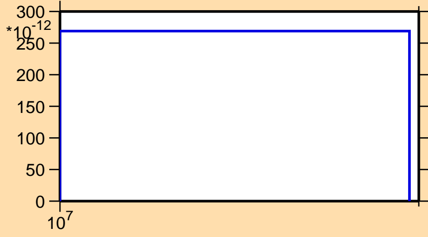
\sigma vs. E for ^{135}\text{Eu}(n,2n\alpha)
