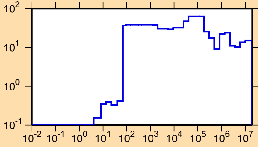
\Delta\sigma/\sigma vs. E for ^{135}\text{Eu}(n,\text{tot.})
