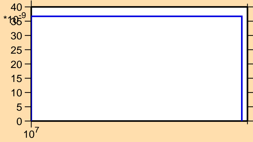
\sigma vs. E for ^{135}\text{Eu}(n,\text{nd})
