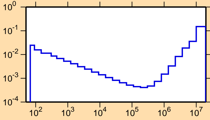
\sigma vs. E for ^{135}\text{Eu}(n,p\alpha)
