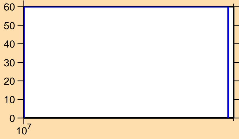
\Delta\sigma/\sigma vs. E for ^{135}\text{Eu}(n,\text{inel.})
