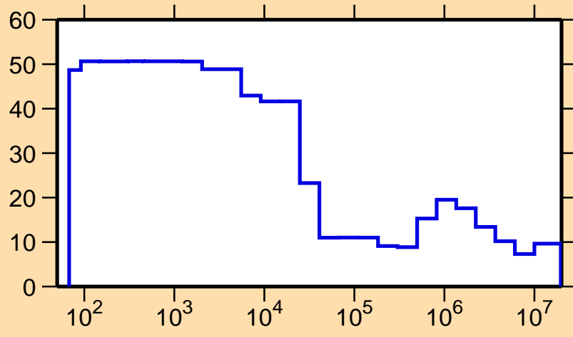
\Delta\sigma/\sigma vs. E for ^{135}\text{Eu}(n,\text{nonel.})
