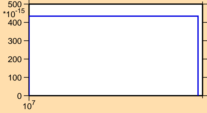
\sigma vs. E for ^{135}\text{Eu}(n,nt)
