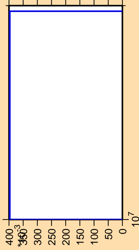
\Delta\sigma/\sigma vs. E for ^{135}\text{Eu}(n,nt)
