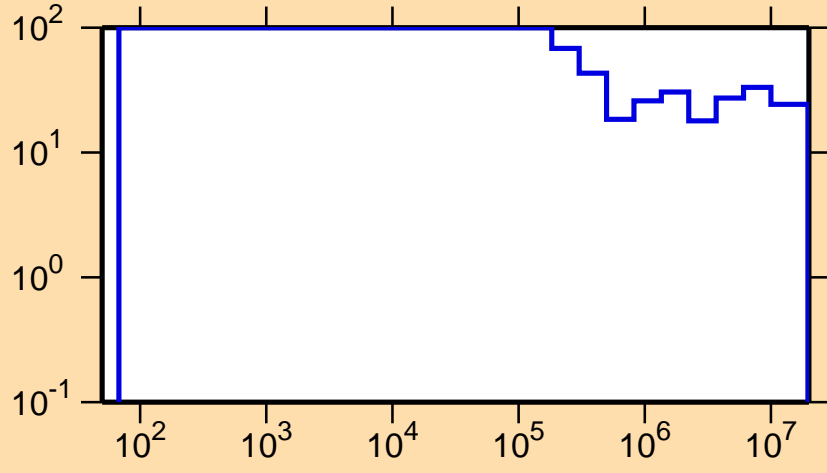
\Delta\sigma/\sigma vs. E for ^{135}\text{Eu}(n,\text{el.})
