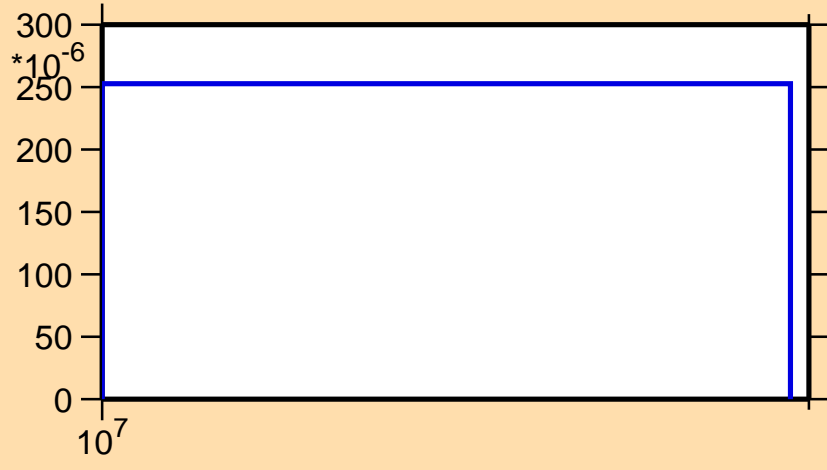
\sigma vs. E for ^{135}\text{Eu}(n,2n)
