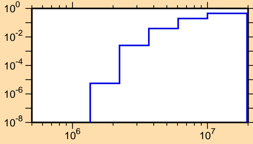
\sigma vs. E for ^{135}\text{Eu}(n,np)
