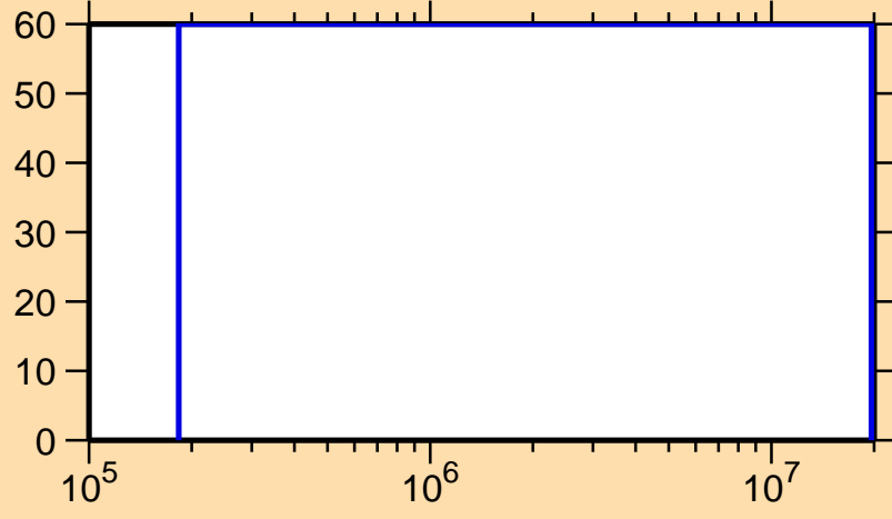
\Delta\sigma/\sigma vs. E for ^{135}\text{Eu}(n,n_1)
