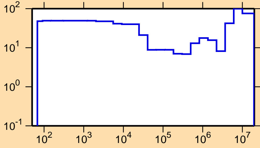
\Delta\sigma/\sigma vs. E for ^{135}\text{Eu}(n,p)
