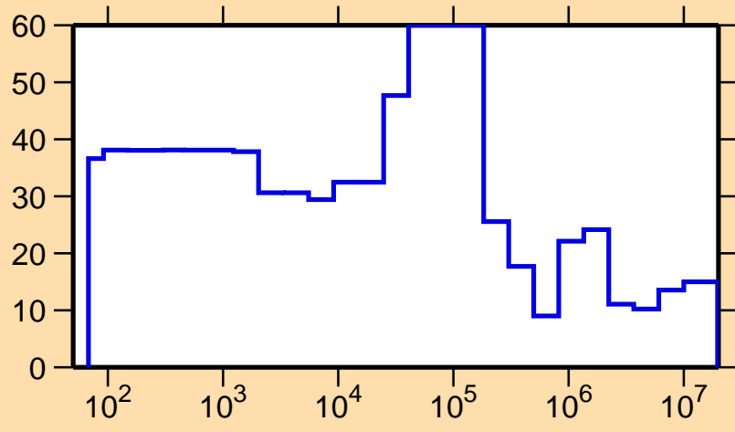
\Delta\sigma/\sigma vs. E for ^{135}\text{Eu}(n,\text{tot.})
