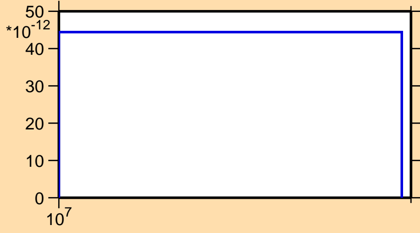
\sigma vs. E for ^{135}\text{Eu} (mt 34)
