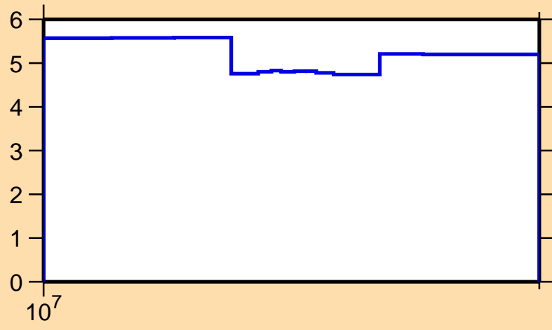
\Delta\sigma/\sigma vs. E for ^{136}\text{Eu}(n,\text{nonel.})
