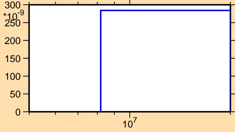
\sigma vs. E for ^{136}\text{Eu}(n,2n\alpha)
