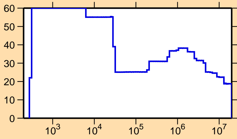
\Delta\sigma/\sigma vs. E for ^{136}\text{Eu}(n,\text{nonel.})
