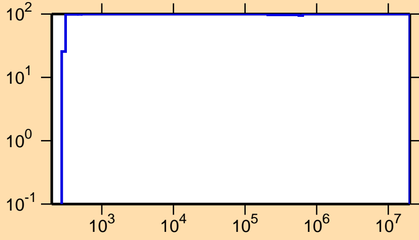
\Delta\sigma/\sigma vs. E for ^{136}\text{Eu}(n,\gamma)
