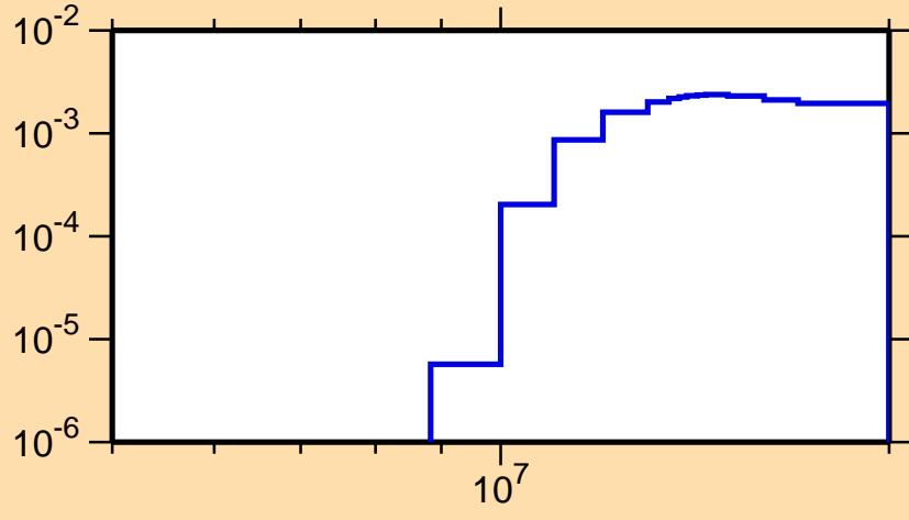
\sigma vs. E for ^{136}\text{Eu}(n,2n)
