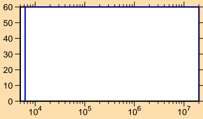
\Delta\sigma/\sigma vs. E for ^{136}\text{Eu}(n,n\text{cont.})
