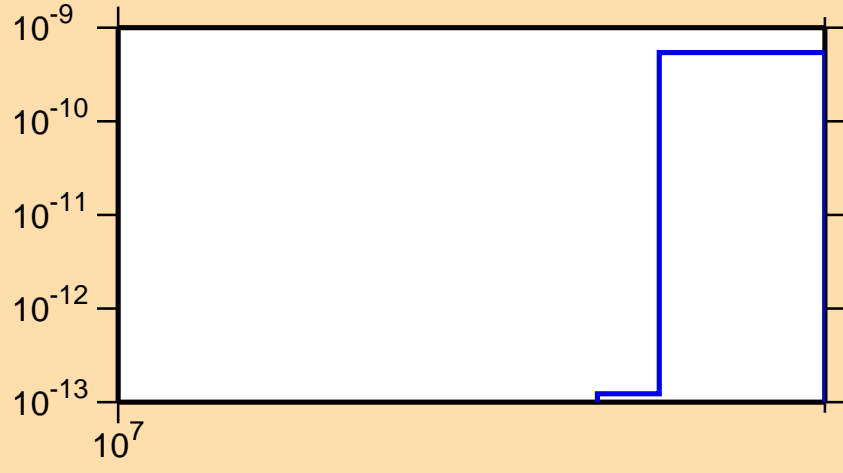
\sigma vs. E for ^{136}\text{Eu}(n,nt)
