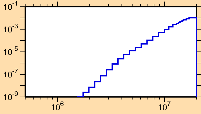
\sigma vs. E for ^{136}\text{Eu}(n,n\alpha)
