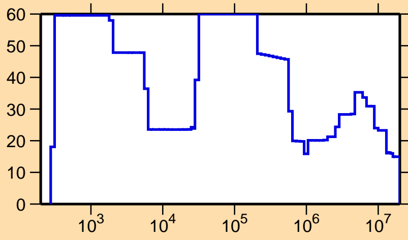
\Delta\sigma/\sigma vs. E for ^{136}\text{Eu}(n,\text{tot.})
