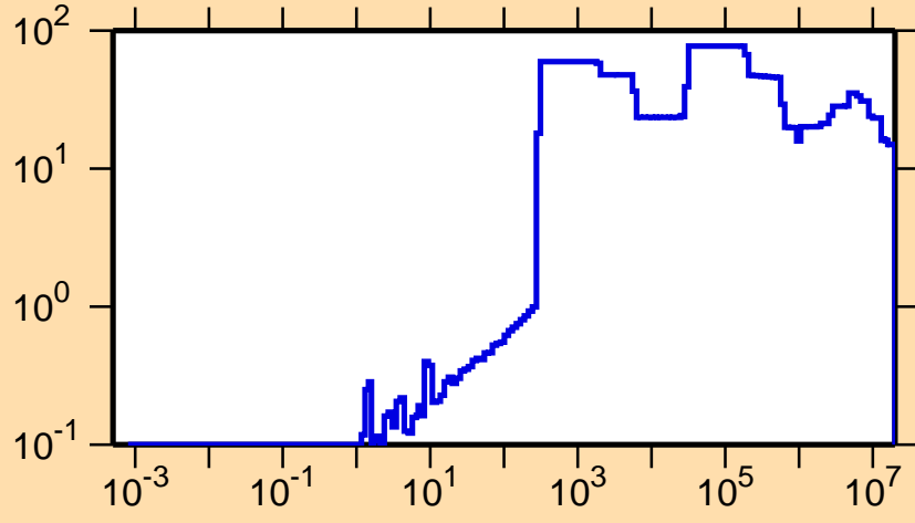
\Delta\sigma/\sigma vs. E for ^{136}\text{Eu}(n,\text{tot.})
