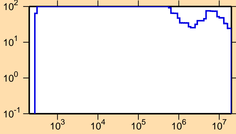
\Delta\sigma/\sigma vs. E for ^{136}\text{Eu}(n,\text{el.})
