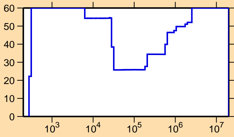
\Delta\sigma/\sigma vs. E for ^{136}\text{Eu}(n,p)
