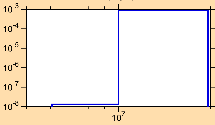
\sigma vs. E for ^{136}\text{Eu}(n,\text{pd})
