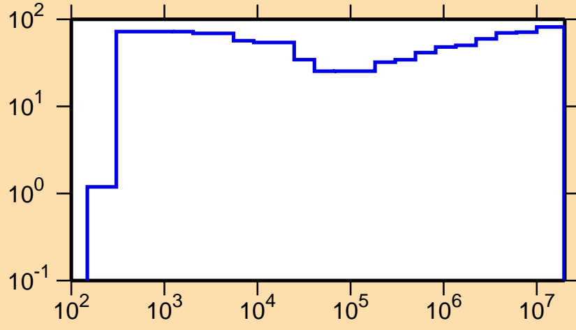
\Delta\sigma/\sigma vs. E for ^{136}\text{Eu}(n,p)
