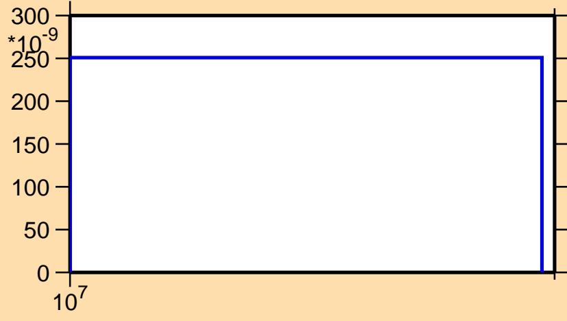
\sigma vs. E for ^{137}\text{Eu}(n,\text{nd})
