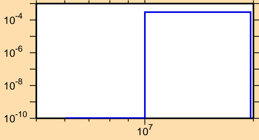
\sigma vs. E for ^{137}\text{Eu}(n,t)
