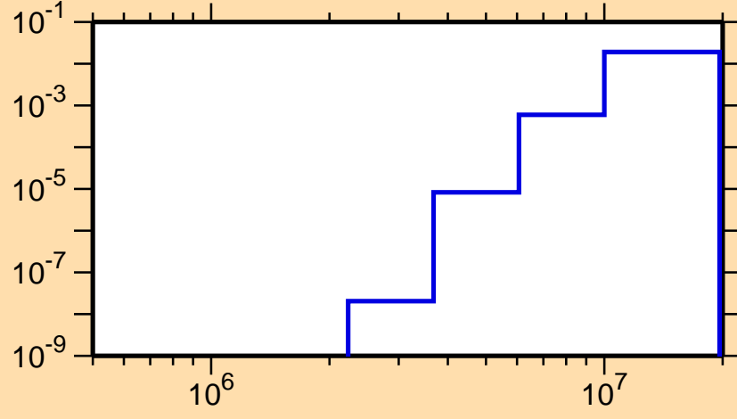
\sigma vs. E for ^{137}\text{Eu}(n,d)
