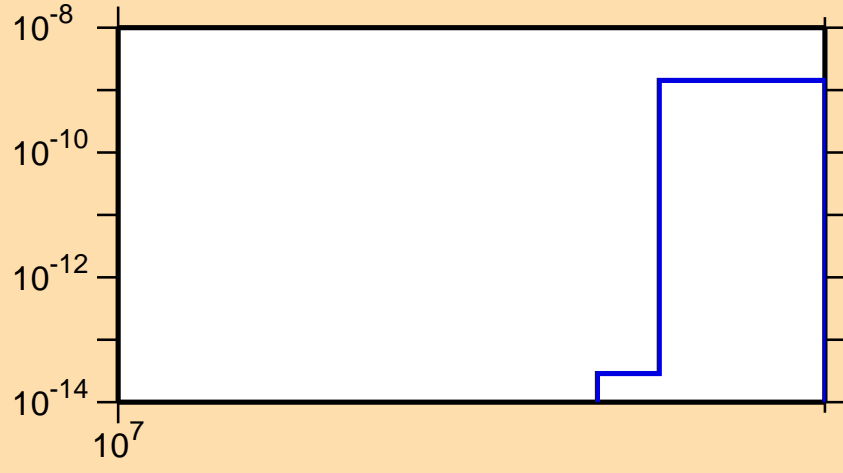
\sigma vs. E for ^{138}\text{Eu}(n,nt)
