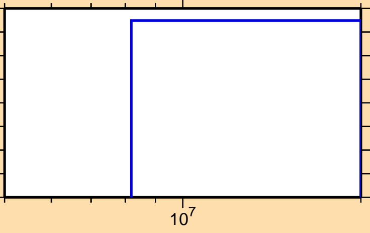
\sigma vs. E for ^{138}\text{Eu}(n,pd)
