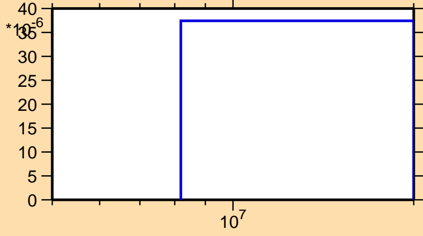
\sigma vs. E for ^{138}\text{Eu}(n,pd)
