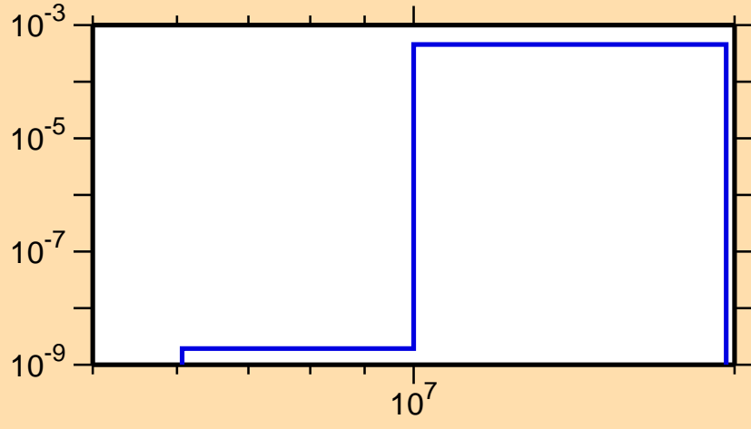
\sigma vs. E for ^{139}\text{Eu}(\text{mt } 45)
